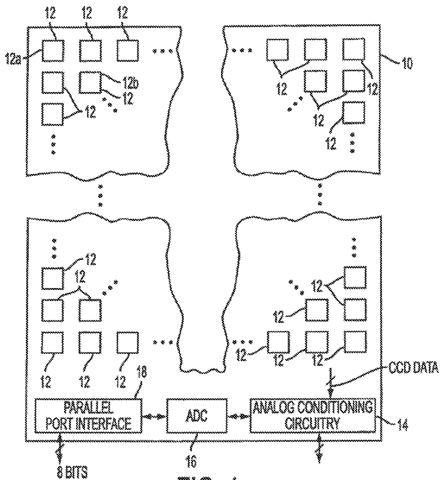
FIG. 1 (PRIOR ART)
