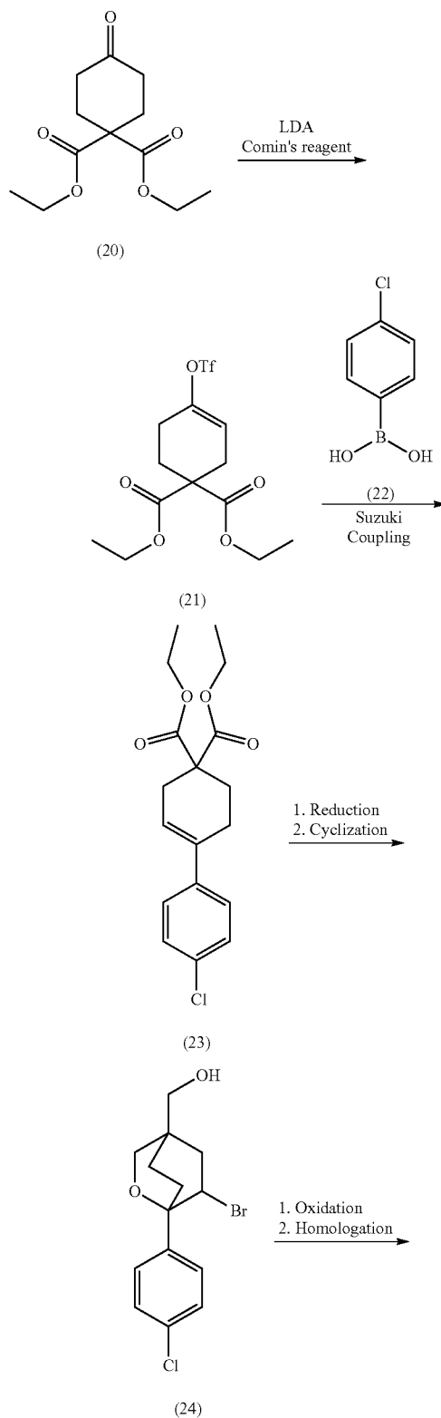
Scheme V: Method of preparing 1-phenyl-2-oxabicyclo[2.2.2]octane compounds
