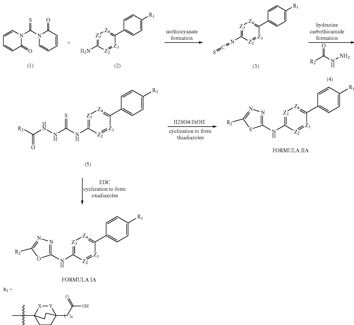
Scheme I: Method of preparing compounds of the invention wherein Ring A is a oxadiazoles or thiadiazoles
