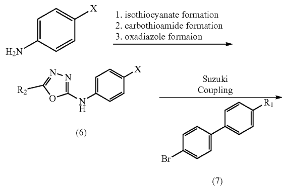
Scheme II: Alternate method of preparing compounds of the invention wherein Ring A is oxadiazole
