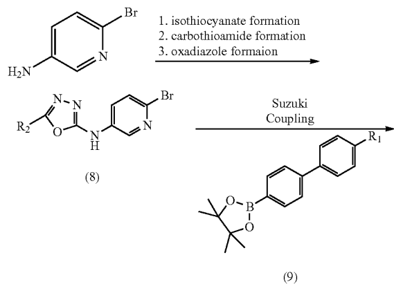
Scheme III: Alternate method of preparing compounds of the invention wherein Ring A is oxadiazole
