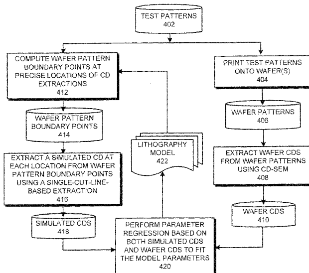
LITHOGRAPHY MODEL CALIBRATION PROCESS 400
