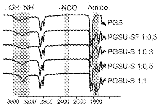
FIG. 6C Wavenumber (cm -1 )
