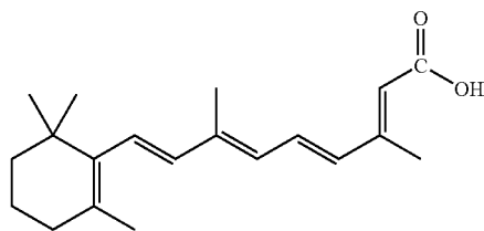
Retinoic Acid (Tretinoin)
