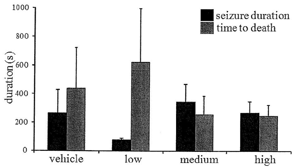
Figure 19: Effects of THCV BDS and 80mg/kg PTZ on seizure duration and time to death
