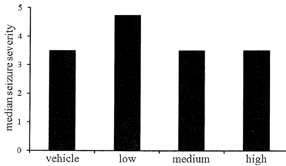
Figure 16: Effects of THCV BDS prior to 70mg/kg PTZ on median severity score
