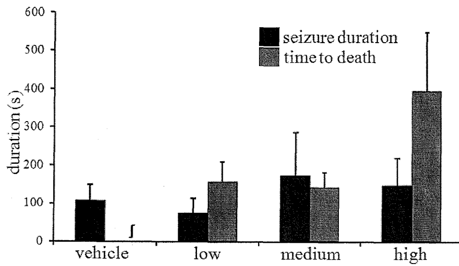
Figure 15: Effects of THCV BDS and 70mg/kg PTZ on seizure duration and time to death
