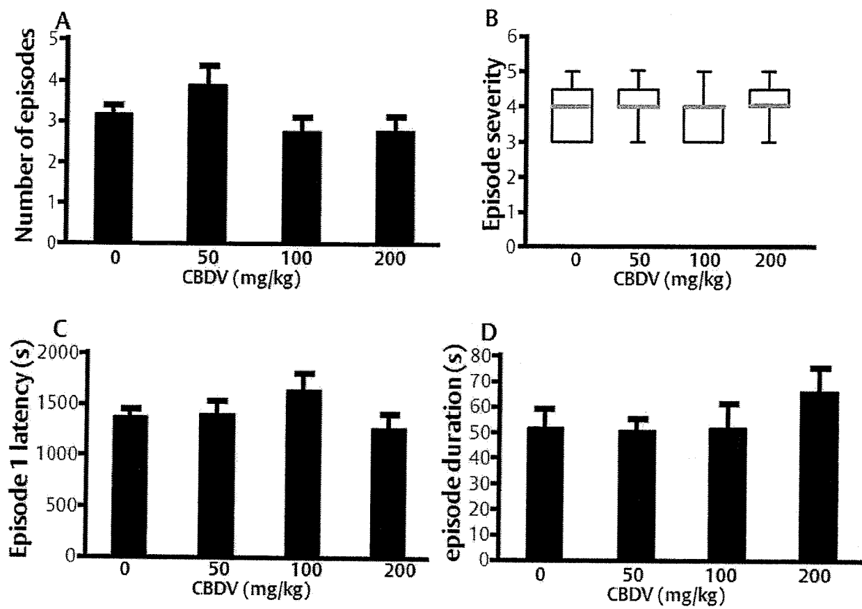
Figure 8: The effect of CBDV on seizure episodes in Pilocarpine-induced seizures;
