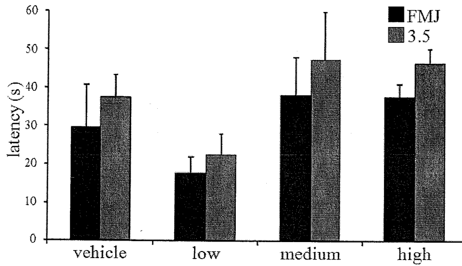
Figure 14 Effects of THCV BDS and 70mg/kg PTZ on latencies to initial and later seizure severities
