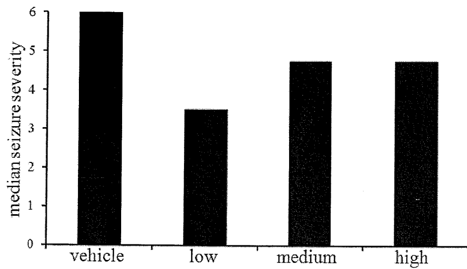
Figure 20: Effects of THCV BDS prior to 80mg/kg PTZ on median severity scores
