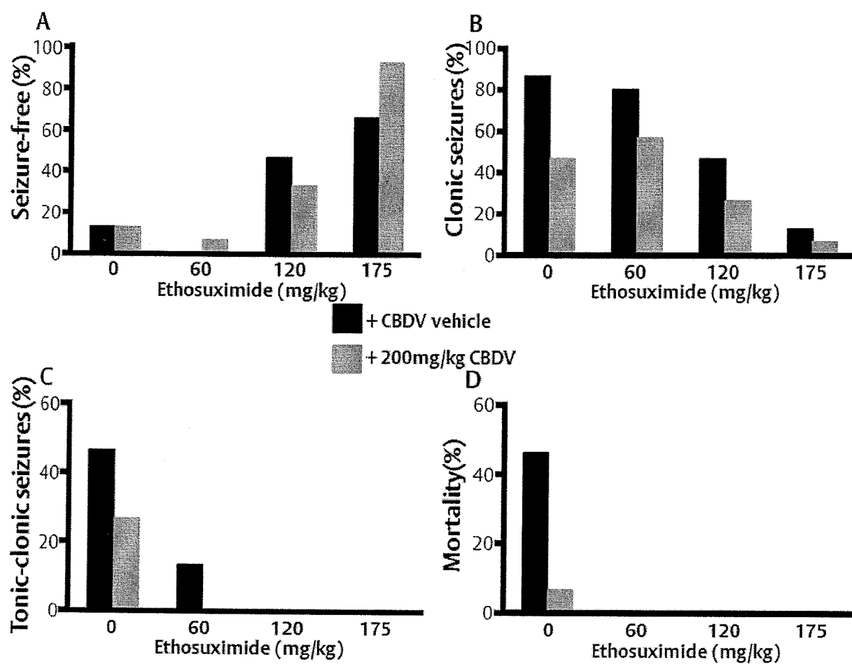
Figure 4: The effect of CBDV and ethosuximide on incidence of seizures and mortality in PTZ-induced seizures
