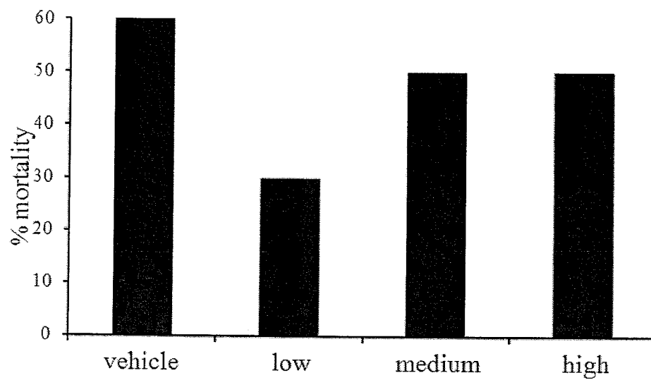
Figure 21: Effects of THCV BDS and 80mg/kg PTZ on mortality rates
