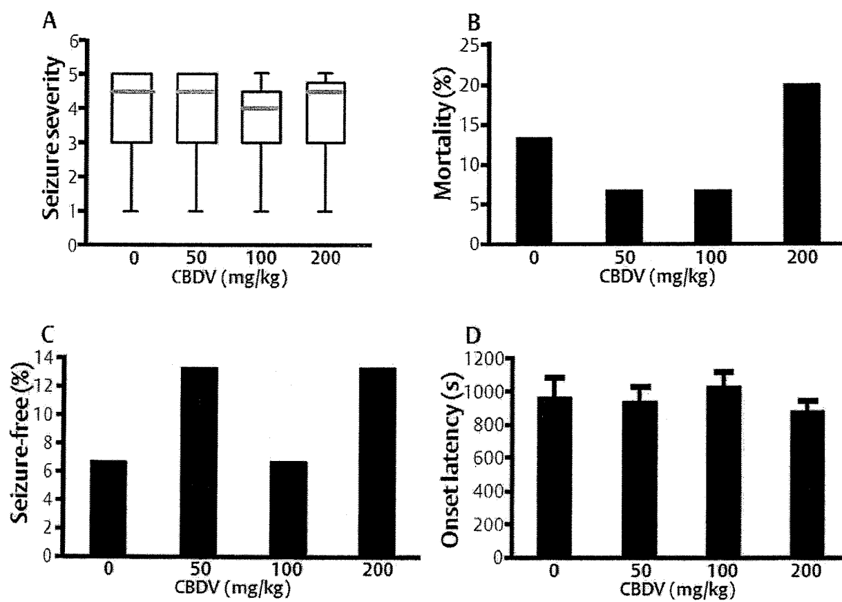
Figure 7: The effect of CBDV in Pilocarpine-induced seizures
