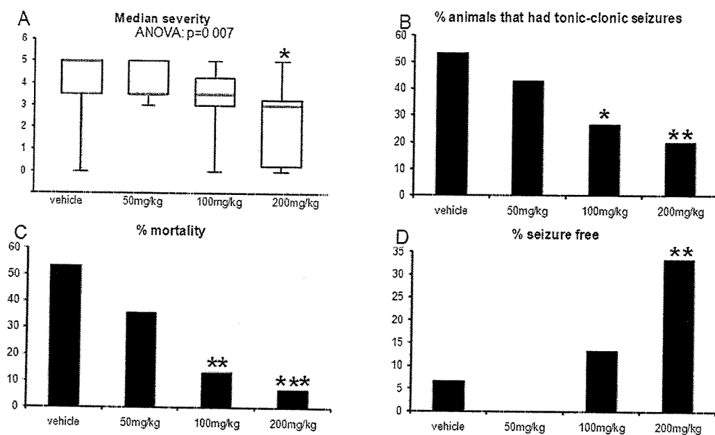
Figure 2: Effects of CBDV on seizure severity and mortality.
