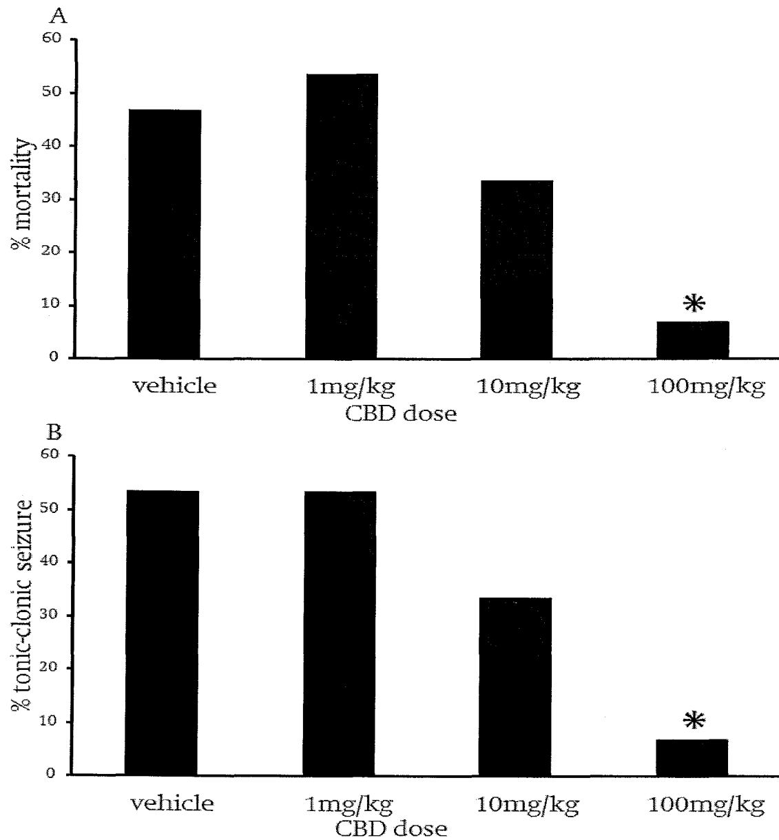
Figure 23 A-B: Effect of CBD on PTZ-induced seizure
