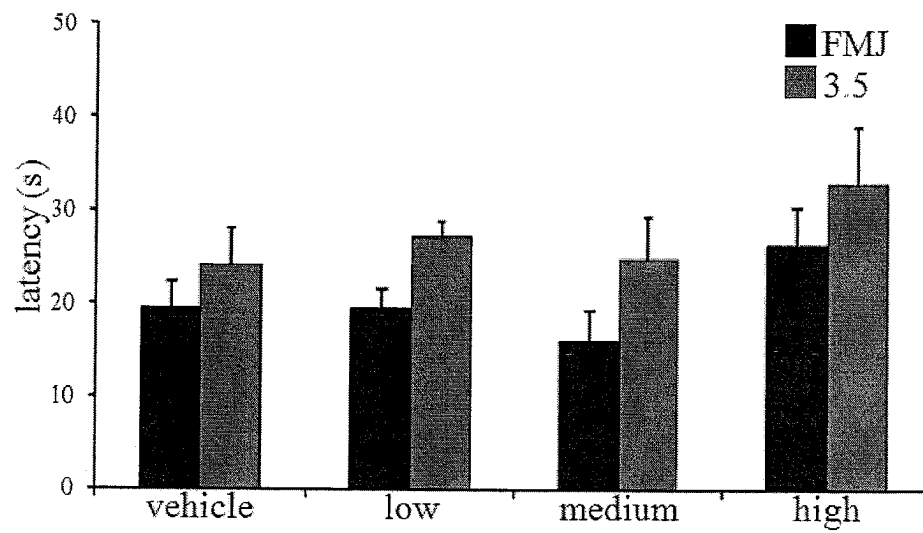
Figure 18: Effects of THCV BDS and 80mg/kg PTZ on latencies to initial and later seizure severities
