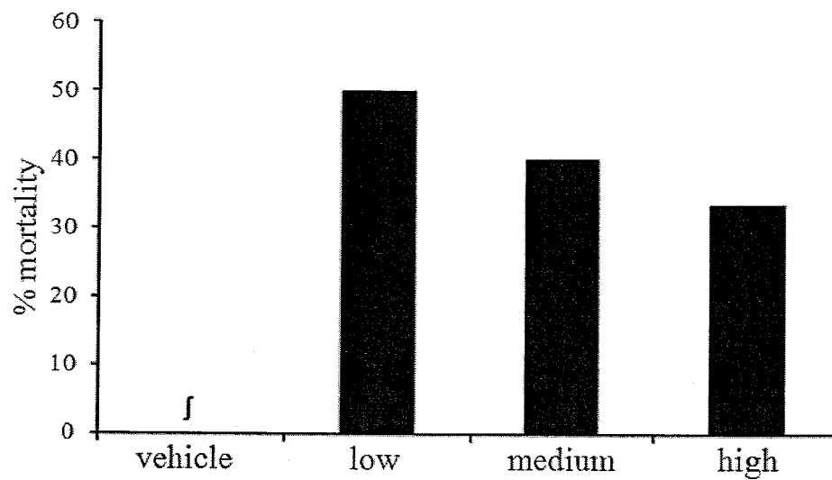
Figure 17: Effects of THCV BDS and 70mg/kg PTZ on mortality rates
