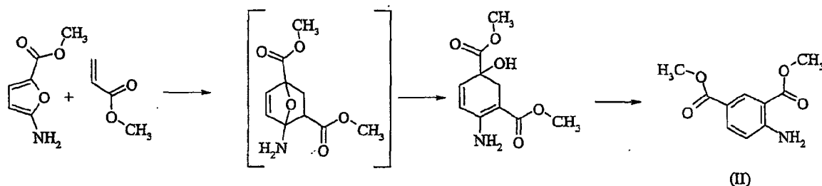
Scheme 3
