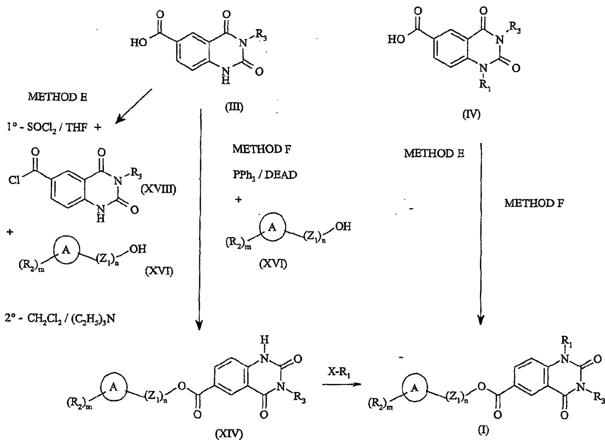
Scheme 8
