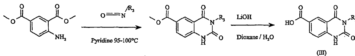
Scheme 4 / Method A
