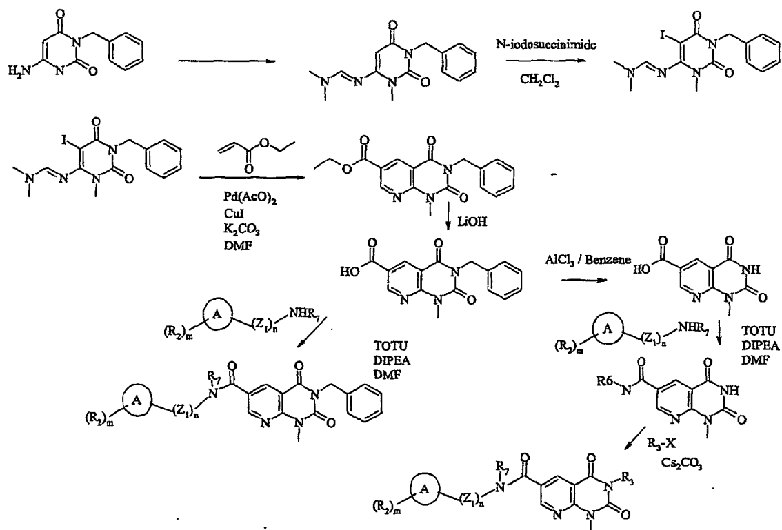
Scheme 10
