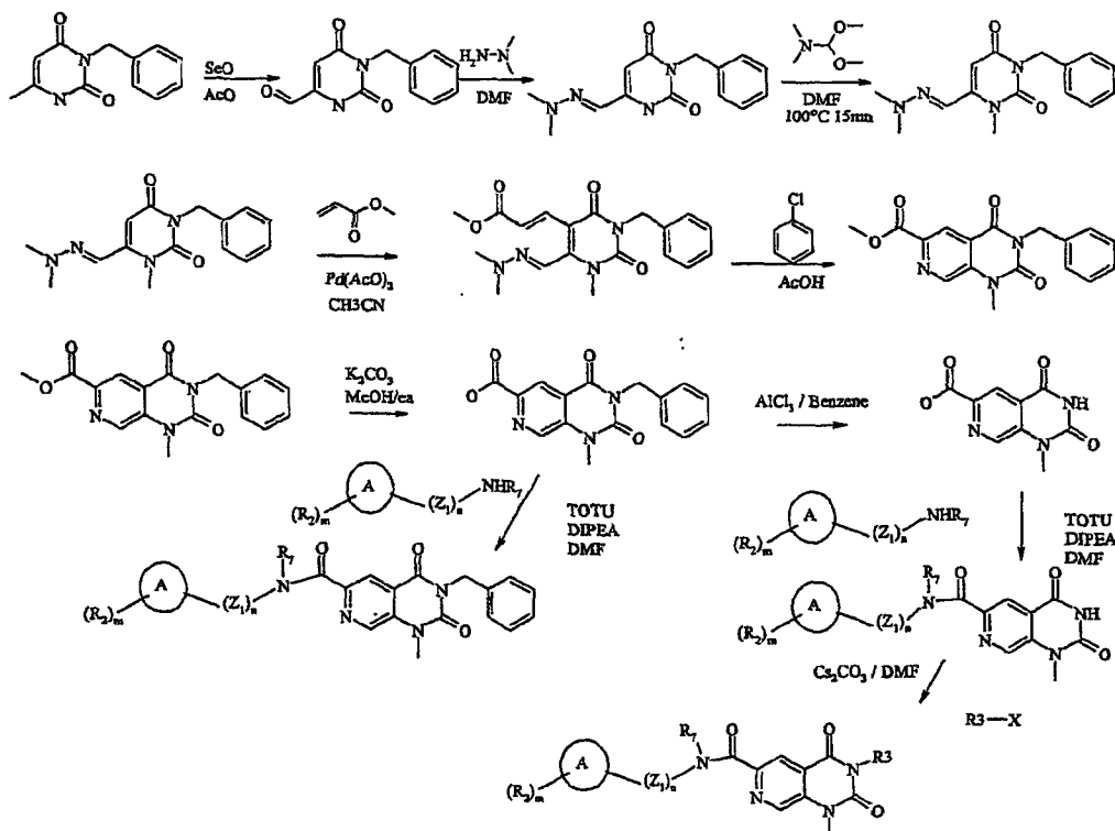
Scheme 11
