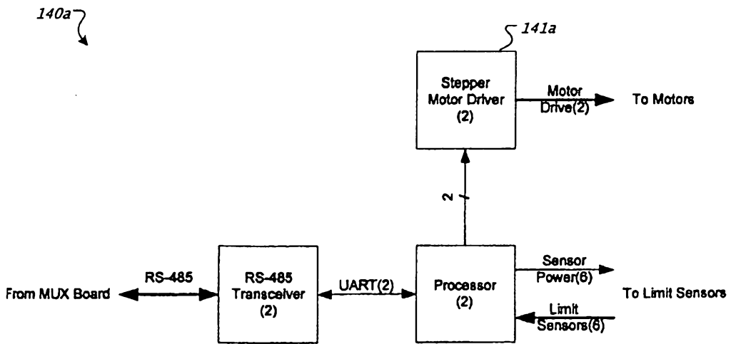
FIG. 91 Motor Control Board Block Diagram
