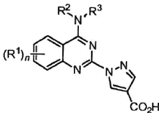
Formel (I)
