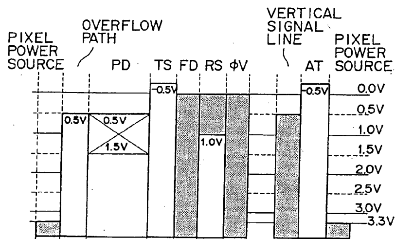
FIG. 4A t < t_1 NON-SELECTION STATE
