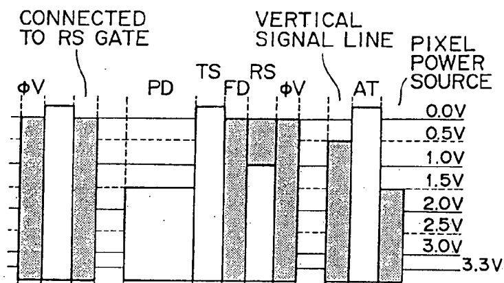
FIG. 13B t_1 < t < t_2 SELECTION
