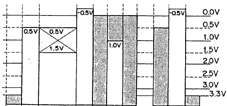
FIG. 5C t_6 < t NON-SELECTION STATE
