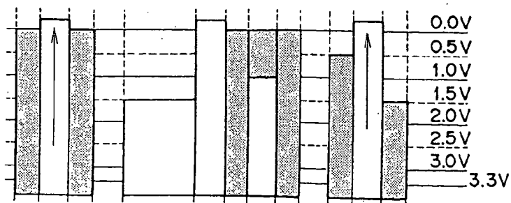
FIG. 14C t_7 < t NON-SELECTION
