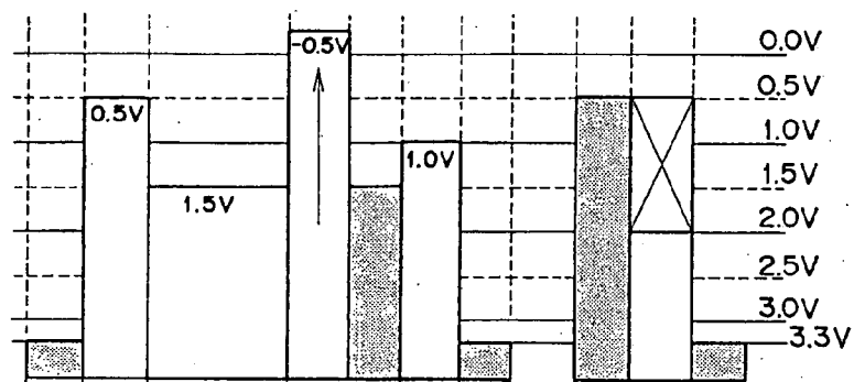
FIG. 5B t_4 < t < t_5 SIGNAL LEVEL READ-OUT
