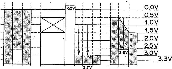
FIG. 13D t_3 < t < t_4 FD RESET
