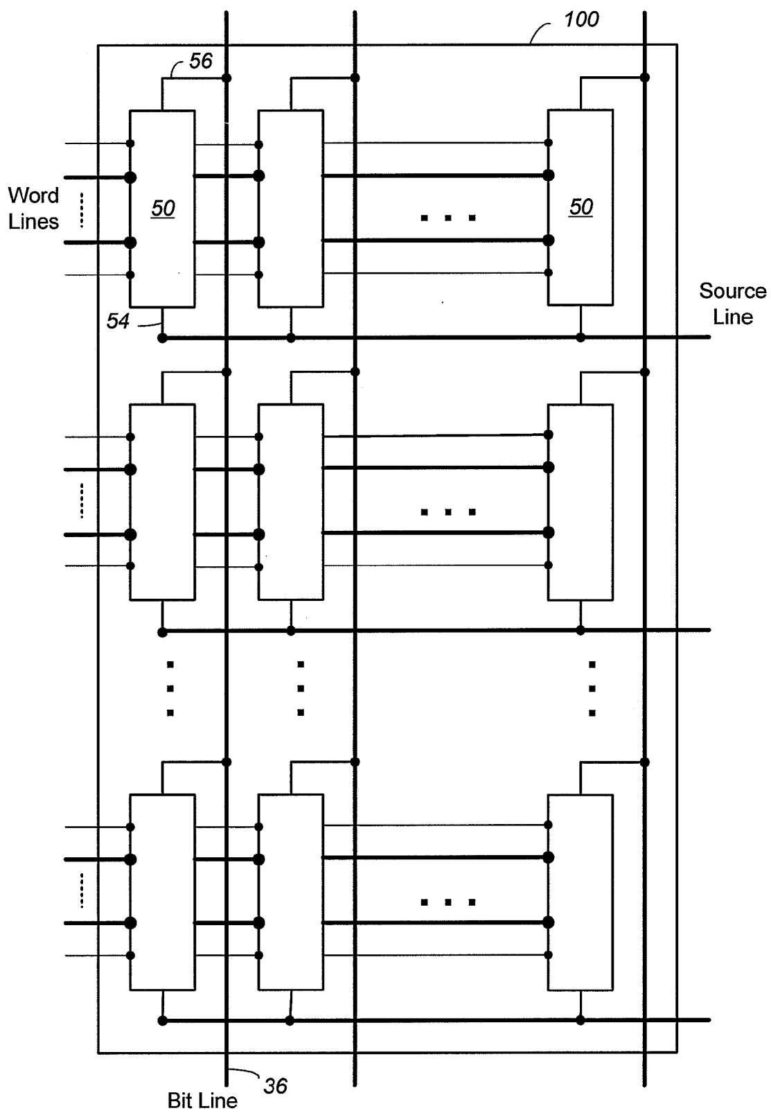
FIG. 3 (Prior Art)
