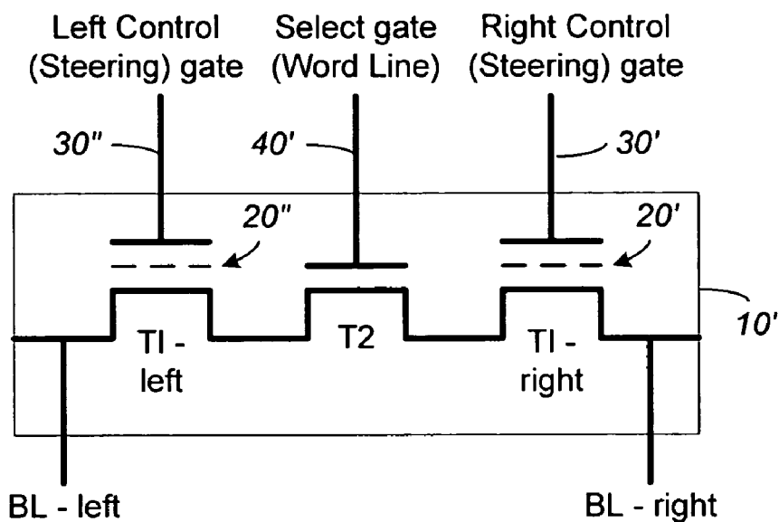
FIG. 1C (Prior Art)
