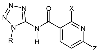
5 Table 4: Compounds of the general formula (I) in which A is N and B is N and W is hydrogen
