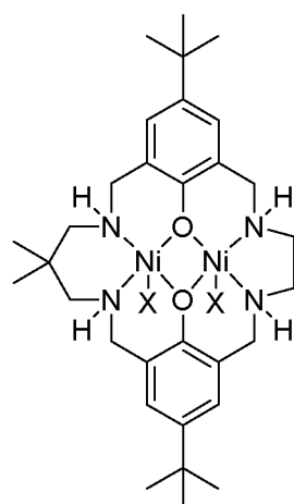
L^{10}Ni_2(OAc)_2
