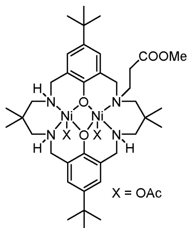
L^{12}Ni_2(OAc)_2
