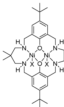
L^{10}Ni_2(OAc)_2
