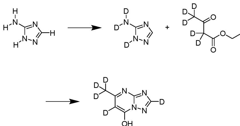
Scheme 3b.
