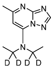
Example 3-1
