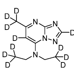
Example 3-8
