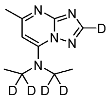
Example 3-4
