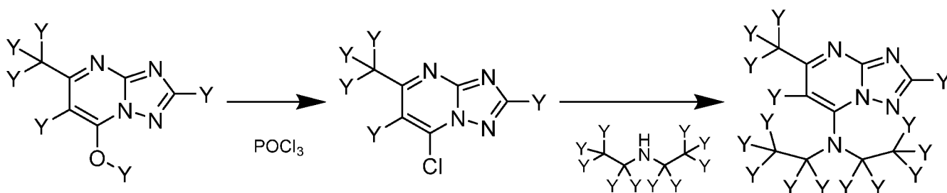
Scheme 2
