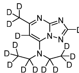
Example 3-9
