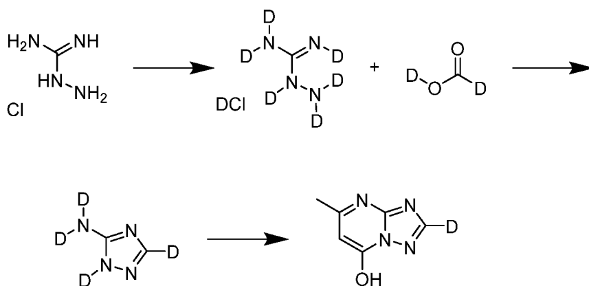
Scheme 3a
