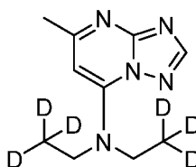
Example 3-2
