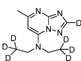
Example 3-5
