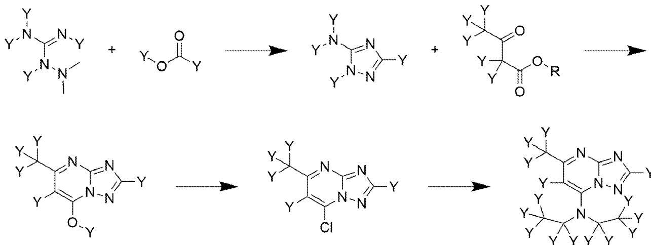
Scheme 1
