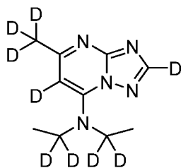
Example 3-7
