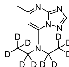
Example 3-3
