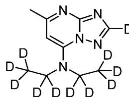
Example 3-6
