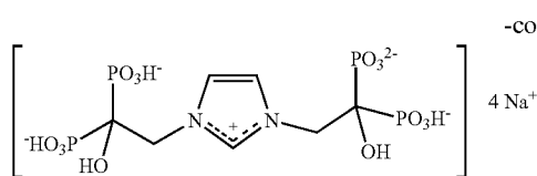
Na salt of Compound 2
