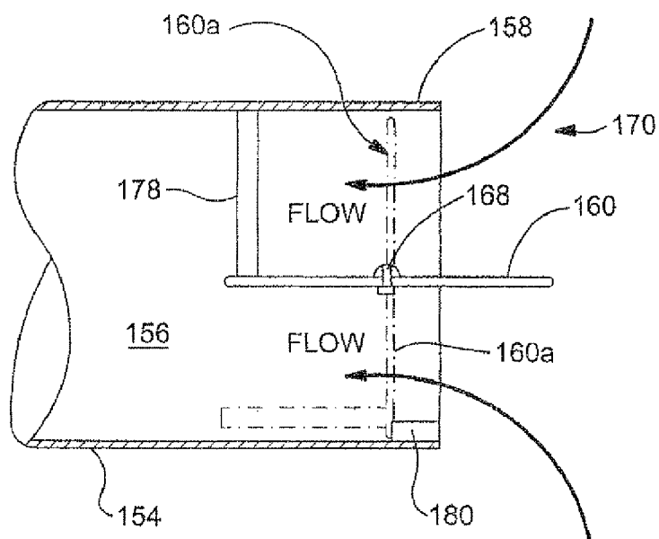
FIG. 8 (PRIOR ART)
