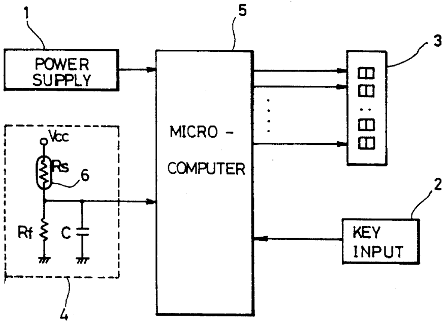
FIG. 1 CONVENTIONAL ART
