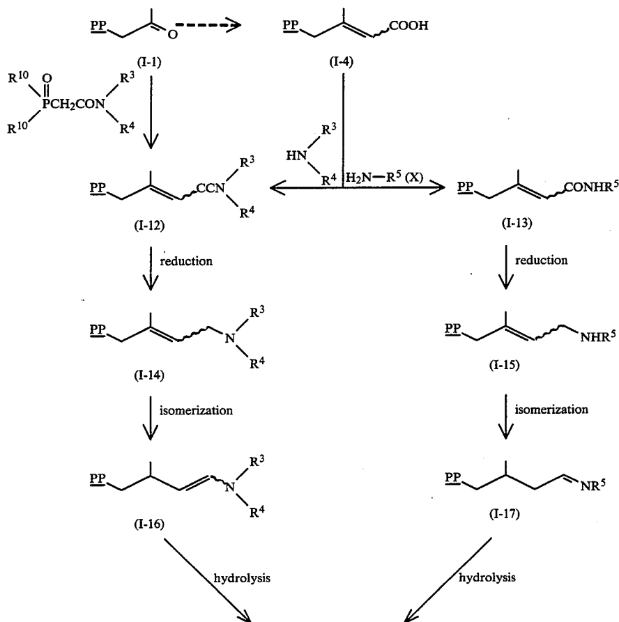
Scheme 3
