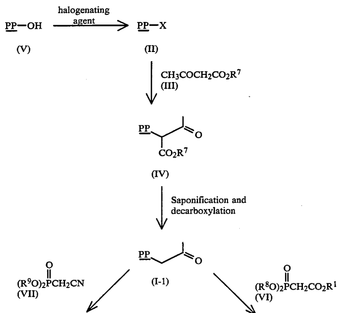
Scheme 1
