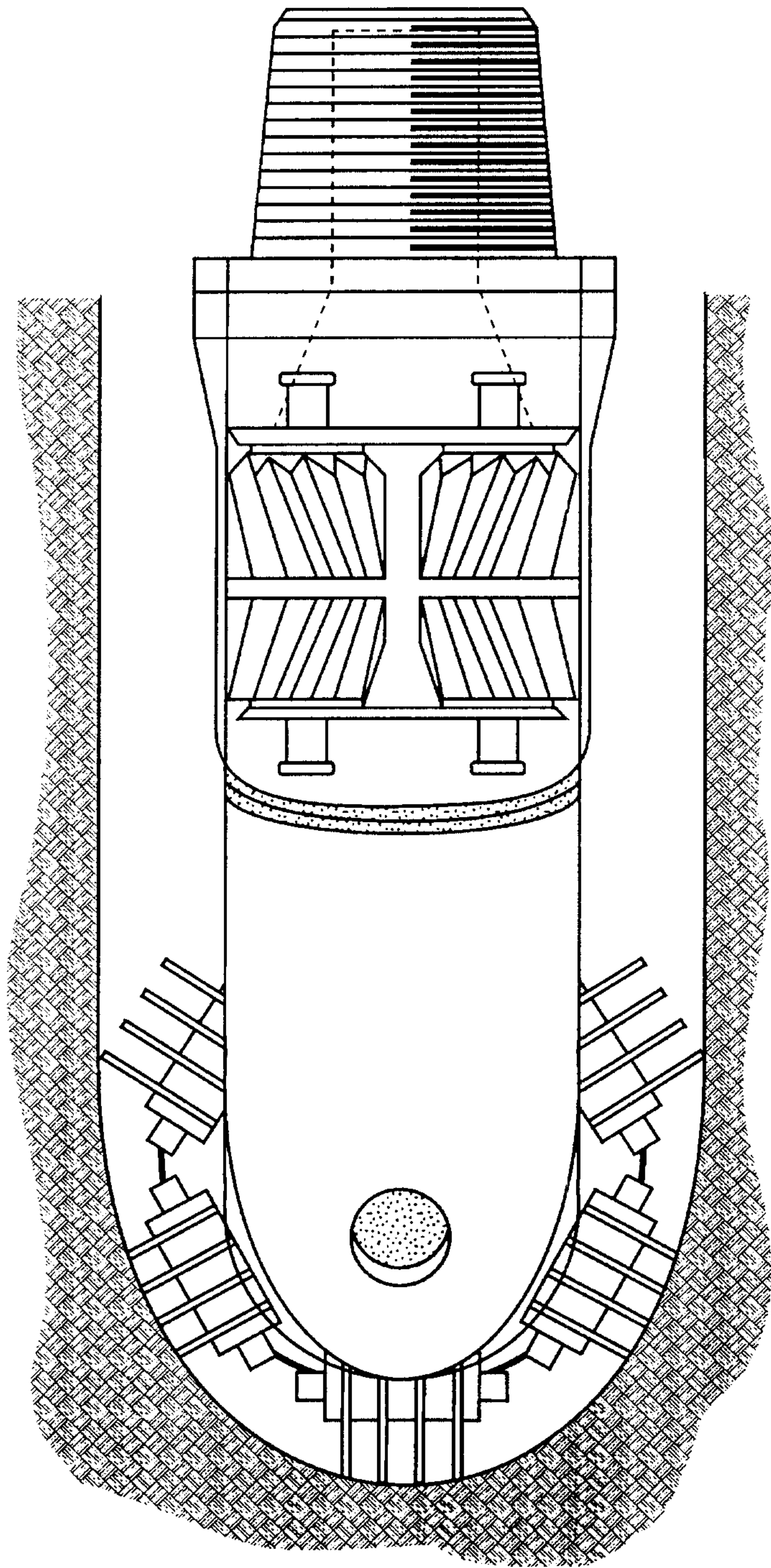
FIG. 1 (Prior Art)
