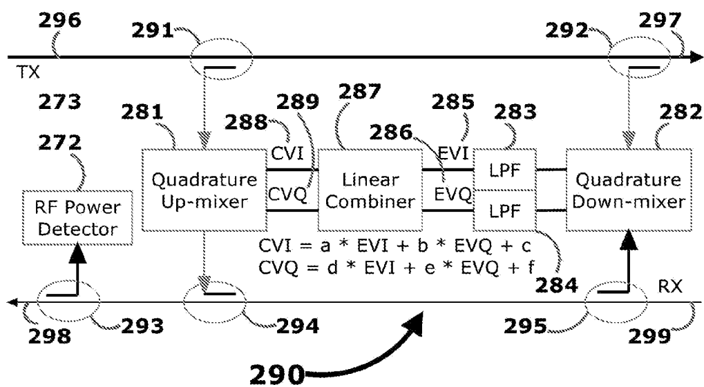
FIG. 2B. Feed-forward transmission leakage canceller.
