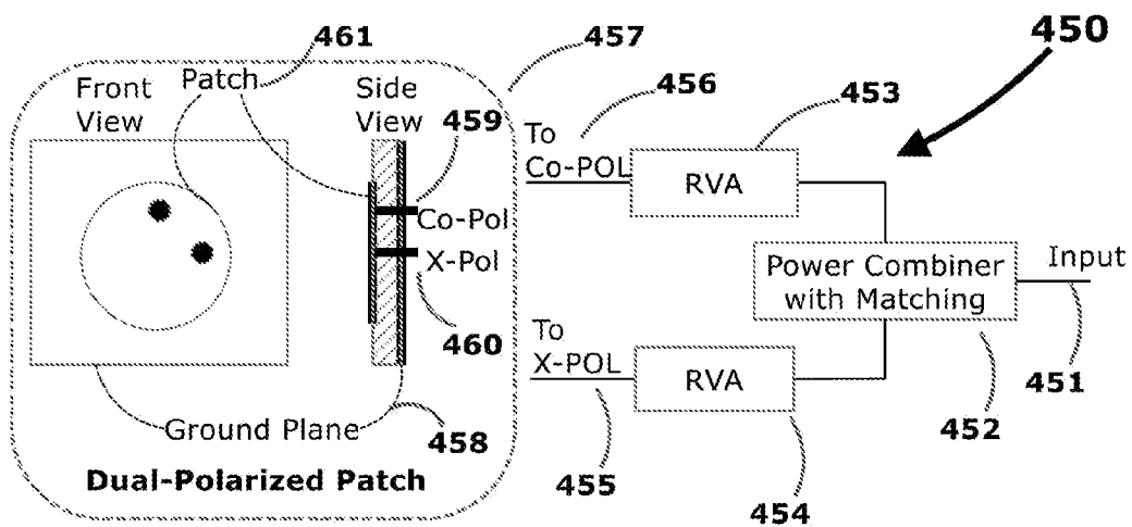
FIG. 4B. Polarization adjustable antenna with matching circuits.
