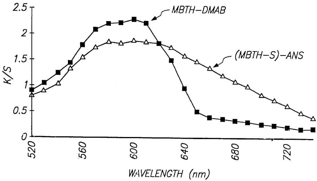
FIG. 1 COMPARISON OF DYE SPECTRA
