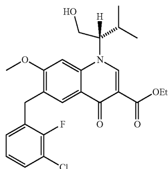
Compound 9a C 25 H 27 ClFNO 5 Mol. Wt.: 475.94
