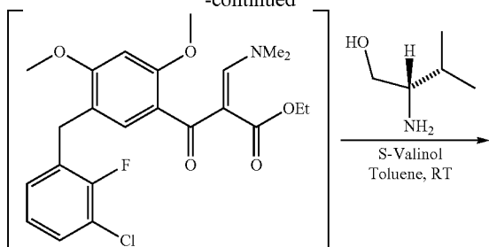
Compound 7a C 23 H 25 ClFNO 5 Mol. Wt.: 449.9
