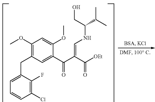
Compound 8a C 26 H 31 ClFNO 6 Mol. Wt.: 507.98
