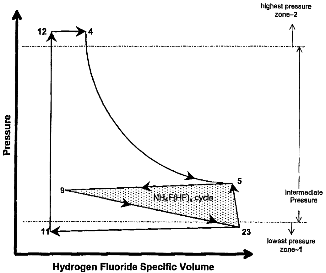
Figure 1. Qualitative pressure-volume plot for Interlocking \text{HF}-\text{NH}_4\text{F}(\text{HF})_x power cycle used to internally generate mechanical energy for mixing \text{F}_2 and \text{NH}_4\text{F}(\text{HF})_x for the production of \text{NF}_3
