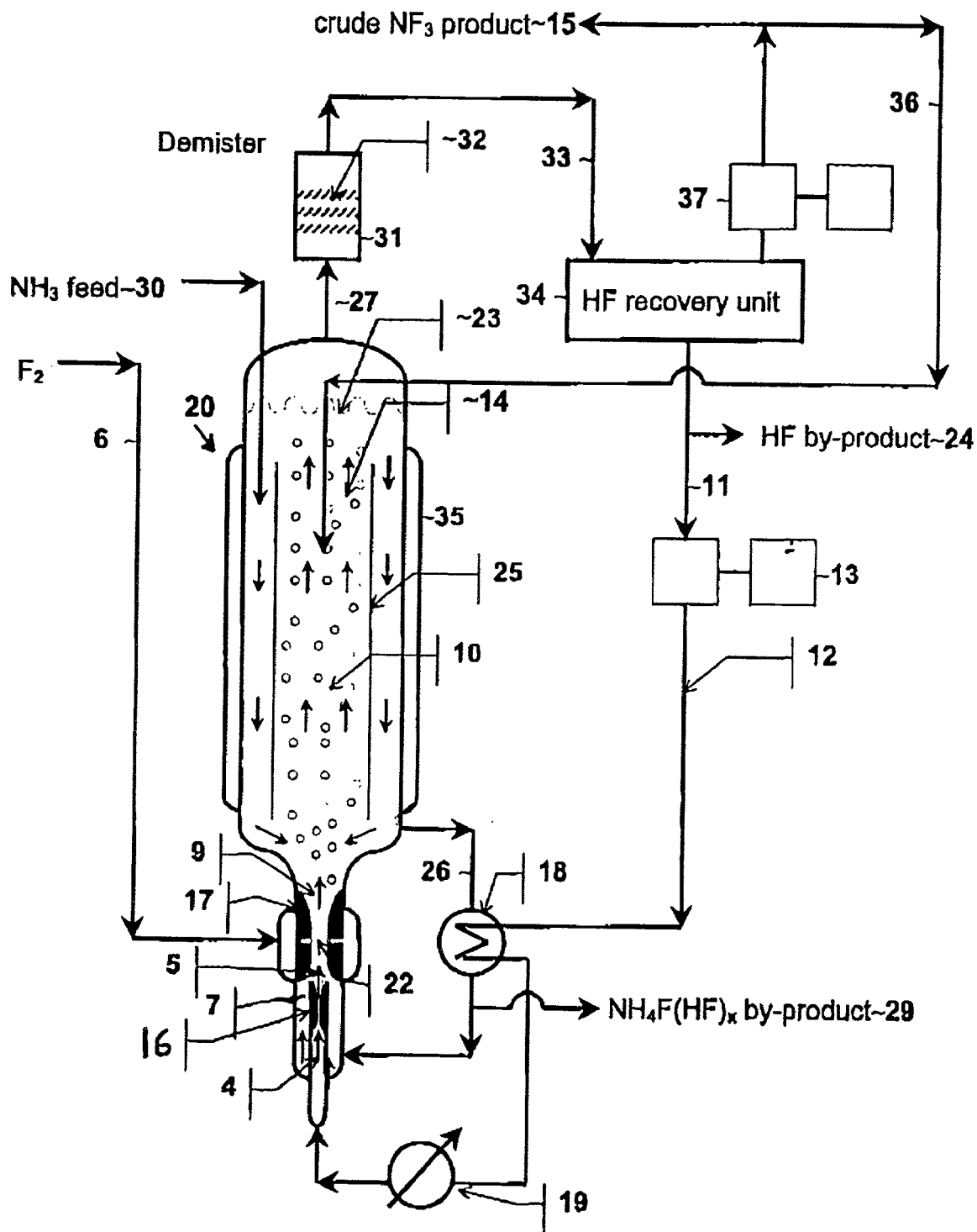
Figure 2. Up-flow reactor using power cycle illustrated on Figure 1 for the production of \text{NF}_3
