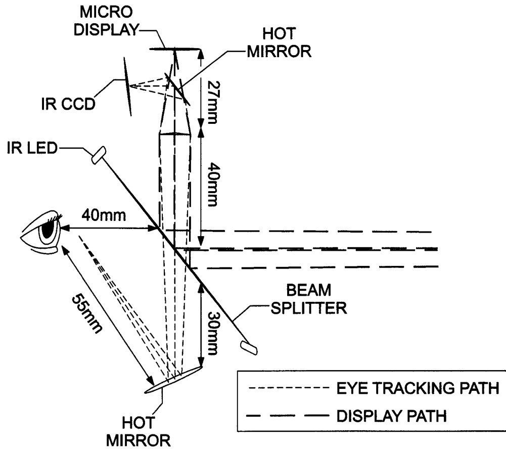
FIG. 1 (PRIOR ART)
