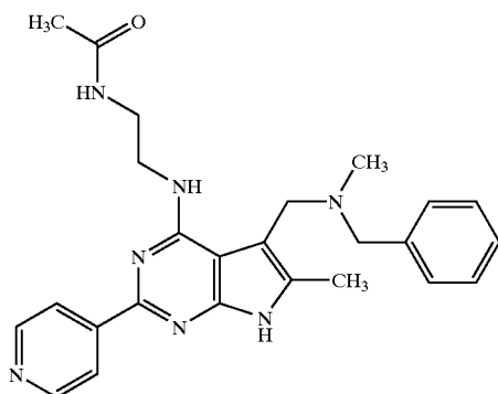
(Compound 1608)
