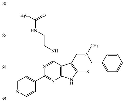
(Compound 1606)
