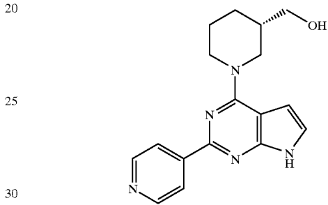
(Compound 1605)
