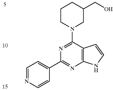
(Compound 1604)
