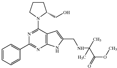
(Compound 1606)
