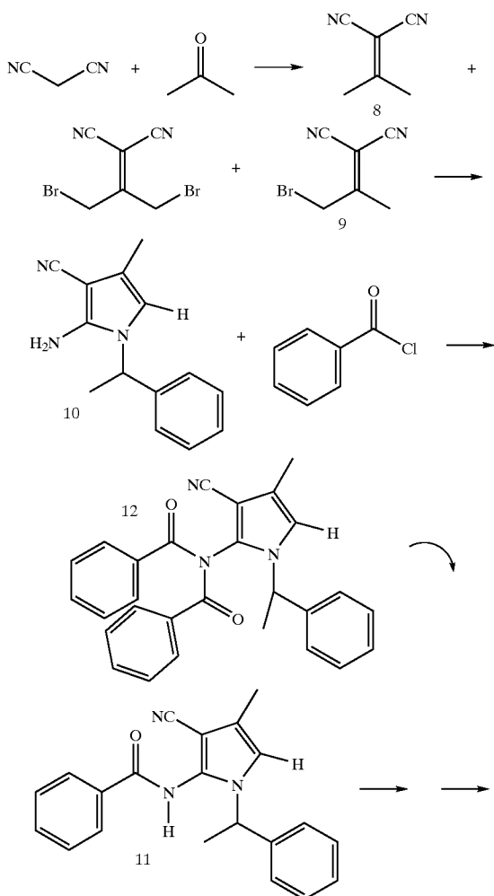
Scheme V
