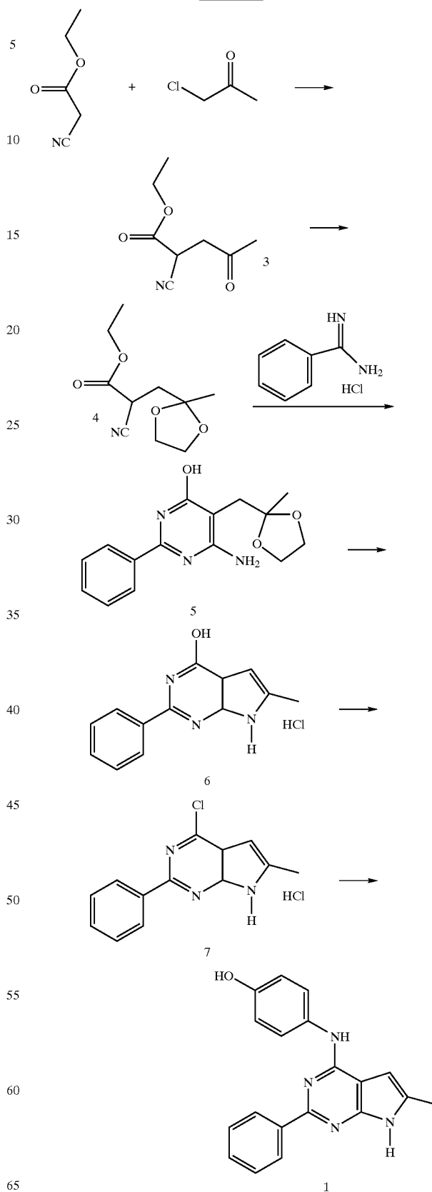
Scheme IV
