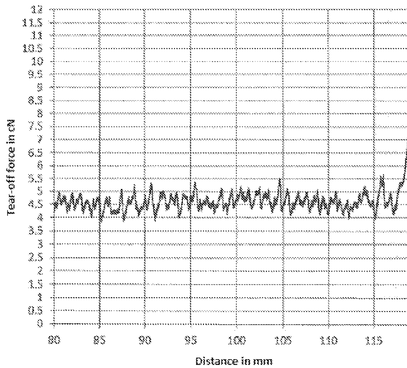
Tear-off force measurement 12 \mu\text{m} carrier
