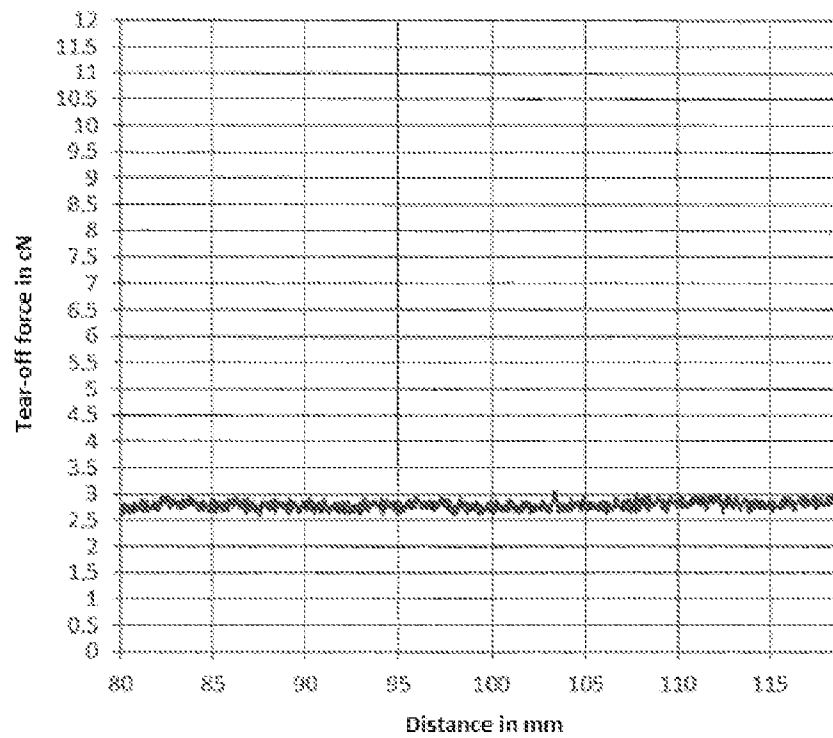
Tear-off force measurement 5.7 \mu\text{m} carrier
