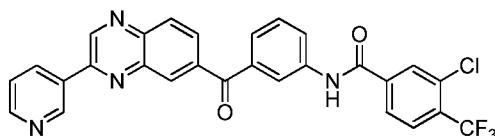
3-chloro- N -(3-(3-(pyridin-3-yl)quinoxaline-6-carbonyl)phenyl)-4-(trifluoromethyl)benzamide
