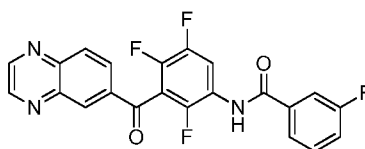
3-fluoro-N-(2,4,5-trifluoro-3-(quinoxaline-6-carbonyl)phenyl)benzamide
