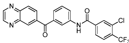
3-chloro- N -(3-(quinoxaline-6-carbonyl)phenyl)-4-(trifluoromethyl)benzamide
