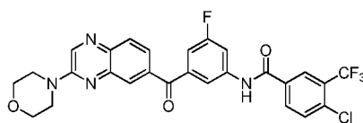
4-chloro-N-(3-fluoro-5-(3-morpholinoquinoxaline-6-carbonyl)phenyl)-3-(trifluoromethyl)benzamide
