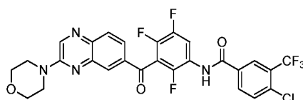
4-chloro-N-(2,4,5-trifluoro-3-(3-morpholinoquinoxaline-6-carbonyl)phenyl)-3-(trifluoromethyl)benzamide
