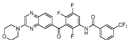
N-(2,4,5-trifluoro-3-(3-morpholinoquinoxaline-6-carbonyl)phenyl)-3-(trifluoromethyl)benzamide
