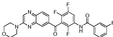
3-fluoro-N-(2,4,5-trifluoro-3-(3-morpholinoquinoxaline-6-carbonyl)phenyl)benzamide
