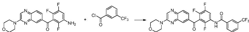
N-(2,4,5-trifluoro-3-(3-morpholinoquinoxaline-6-carbonyl)phenyl)-3-(trifluoromethyl)benzamide
