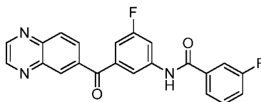
3-fluoro-N-(3-fluoro-5-(quinoxaline-6-carbonyl)phenyl)benzamide
