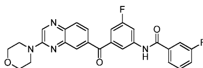
3-fluoro-N-(3-fluoro-5-(3-morpholinoquinoxaline-6-carbonyl)phenyl)benzamide
