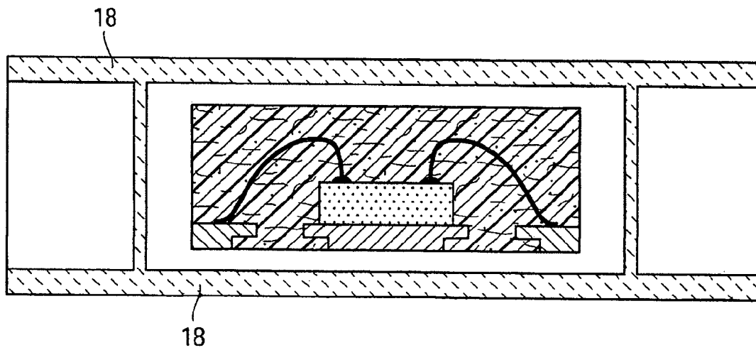
FIG 1K (PRIOR ART)
