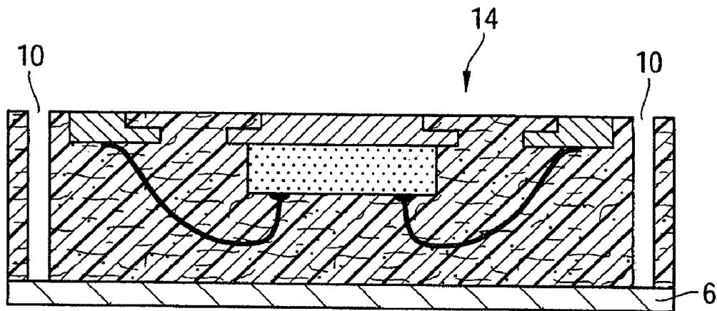
FIG 1H (PRIOR ART)
