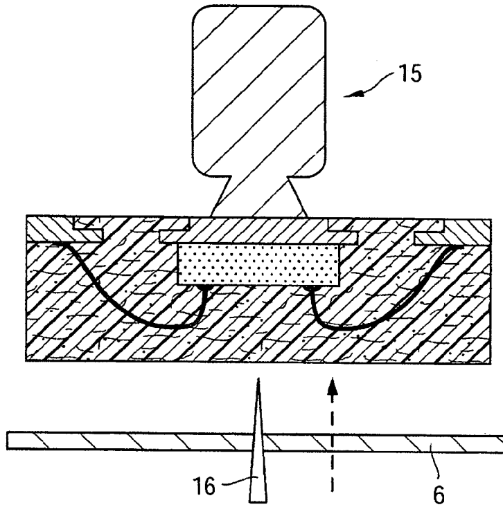
FIG 1J (PRIOR ART)
