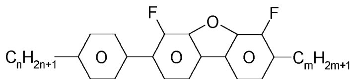
PB-n-m
