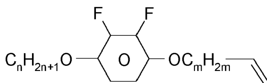
Y-nO-OmV
