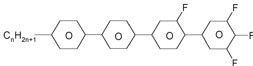
PPGU-n-F
