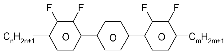
YPY-n-m
