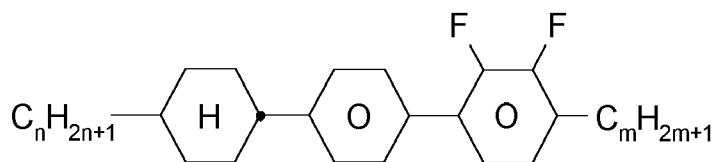
CPY-n-m
