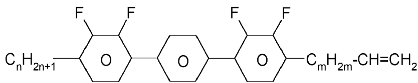
YPY-n-mV
