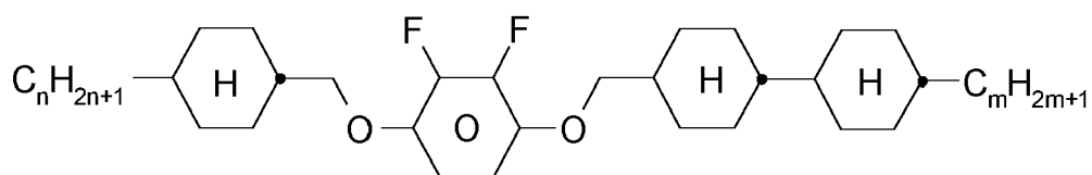
COYOICC-n-m
