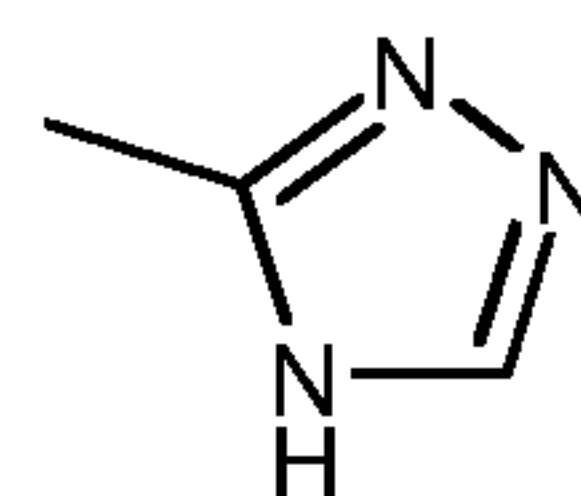
4H-tautomer.
