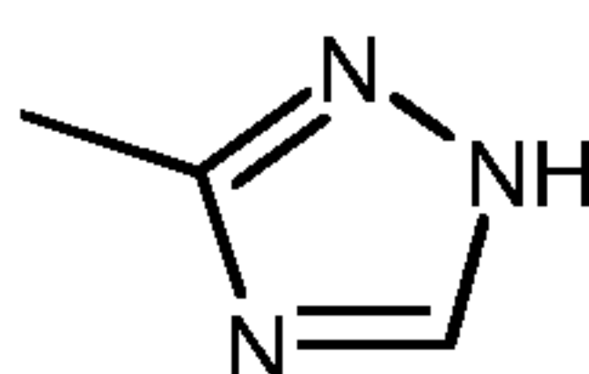
2H-tautomer
