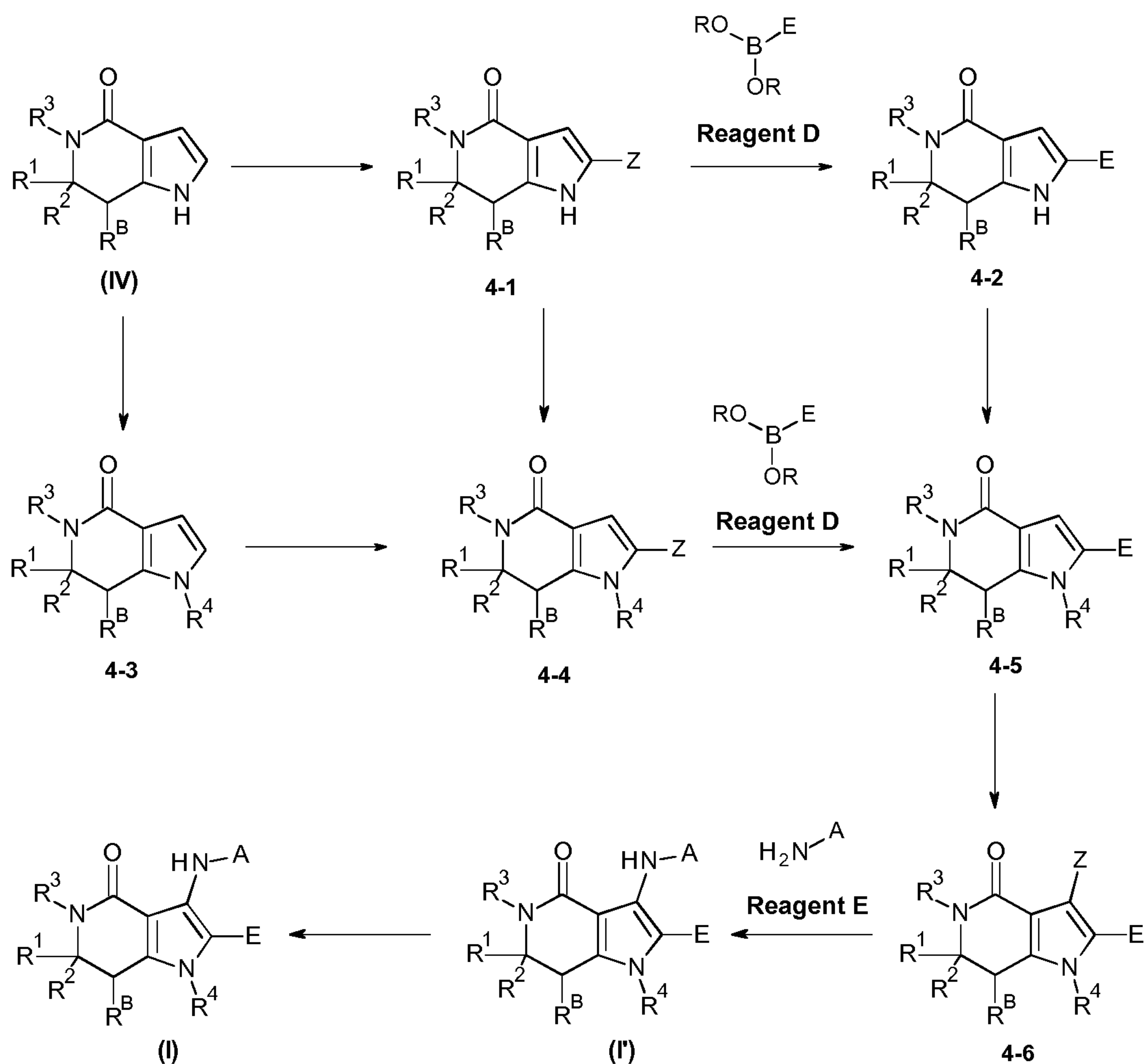
Scheme 4
