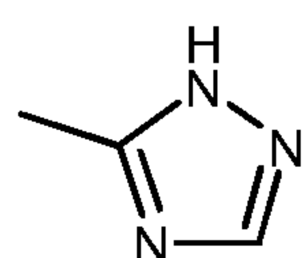
1H-tautomer
