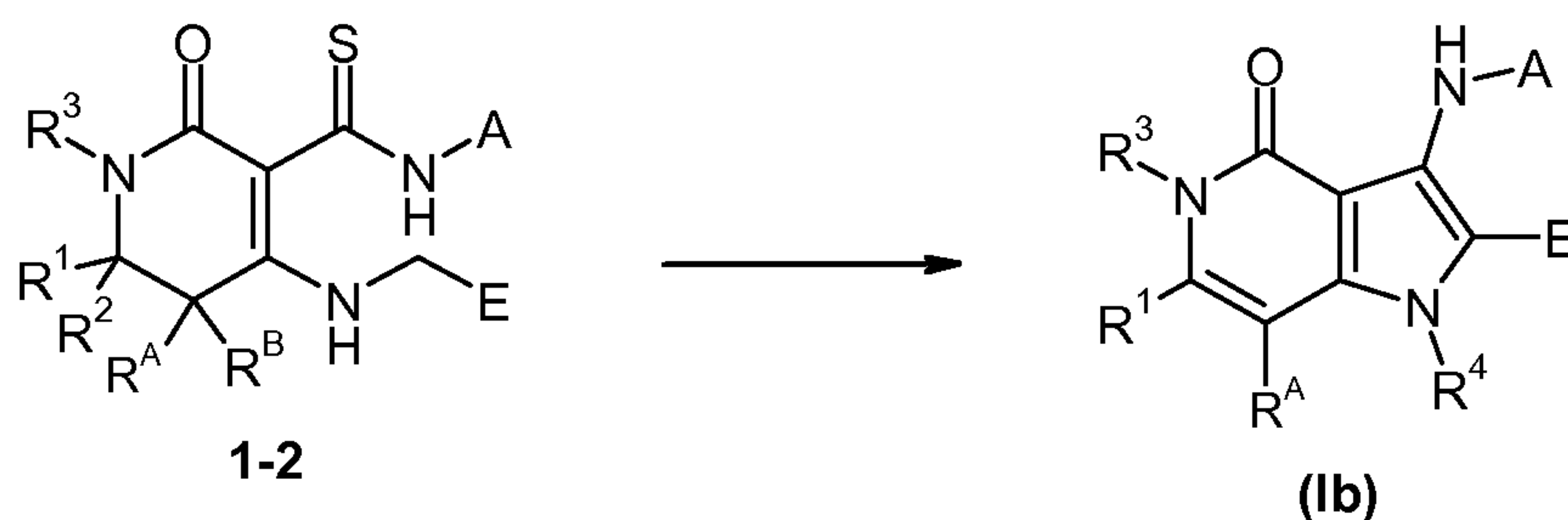
Scheme 2
