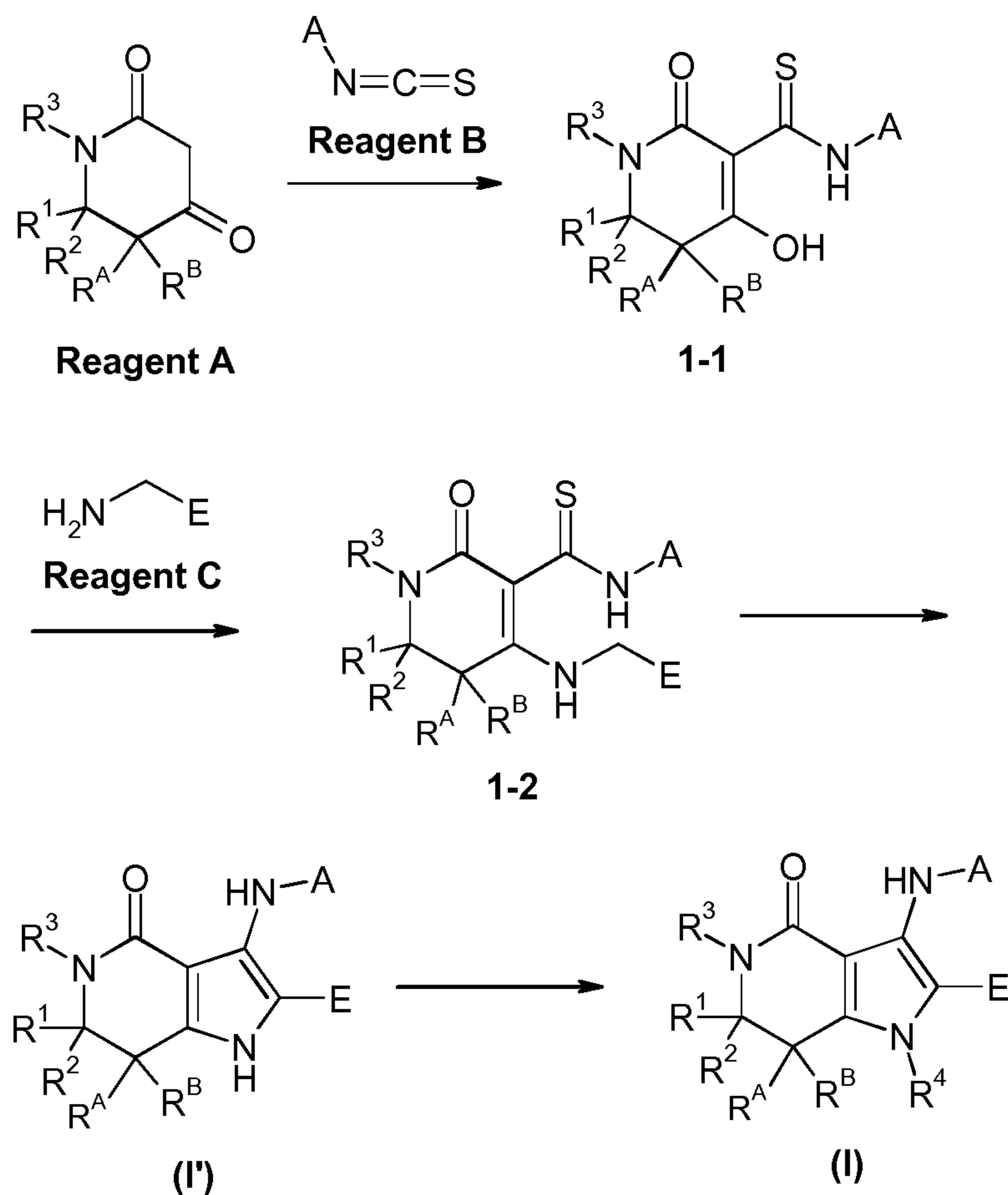
Scheme 1
