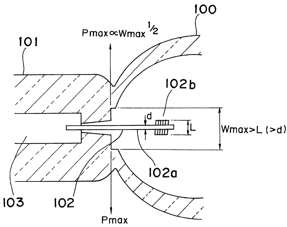
Fig. 9 PRIOR ART
