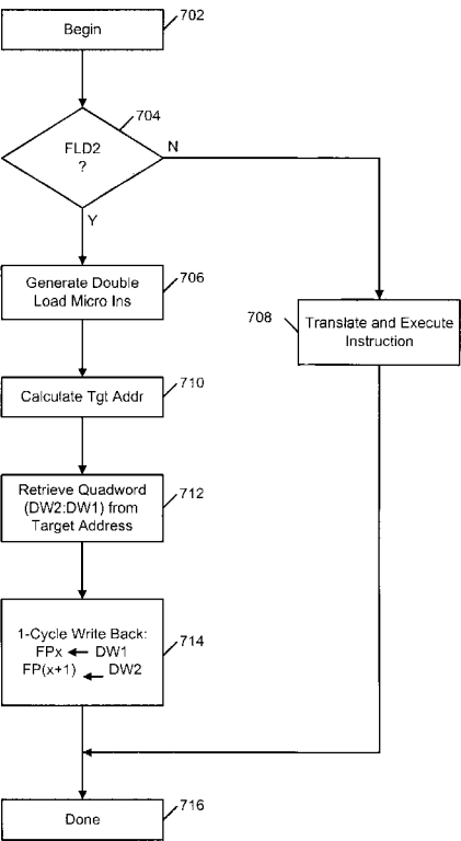
Method for Double Operand Load
