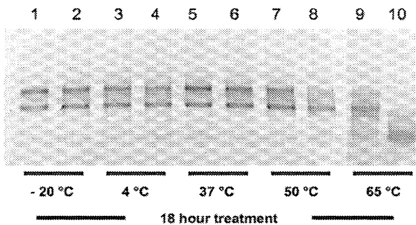
Figure 3. RNA stabilisation in Choline chloride:Urea at a range of temperatures.
