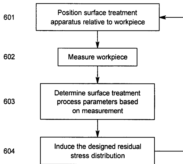
FIG. 6: Flow diagram of one embodiment of the method of performing a surface treatment operation
