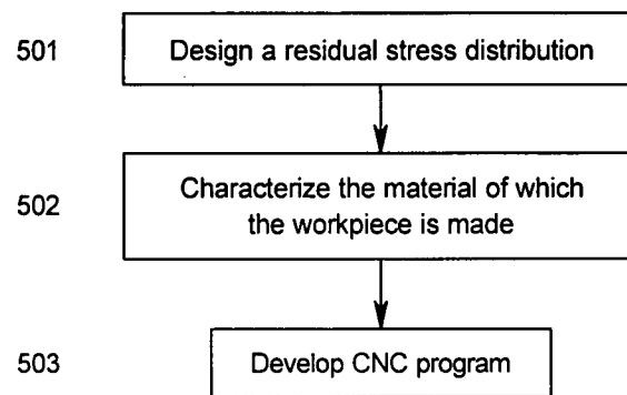
FIG. 5 preliminary steps to one embodiment of the method of performing a surface treatment operation.
