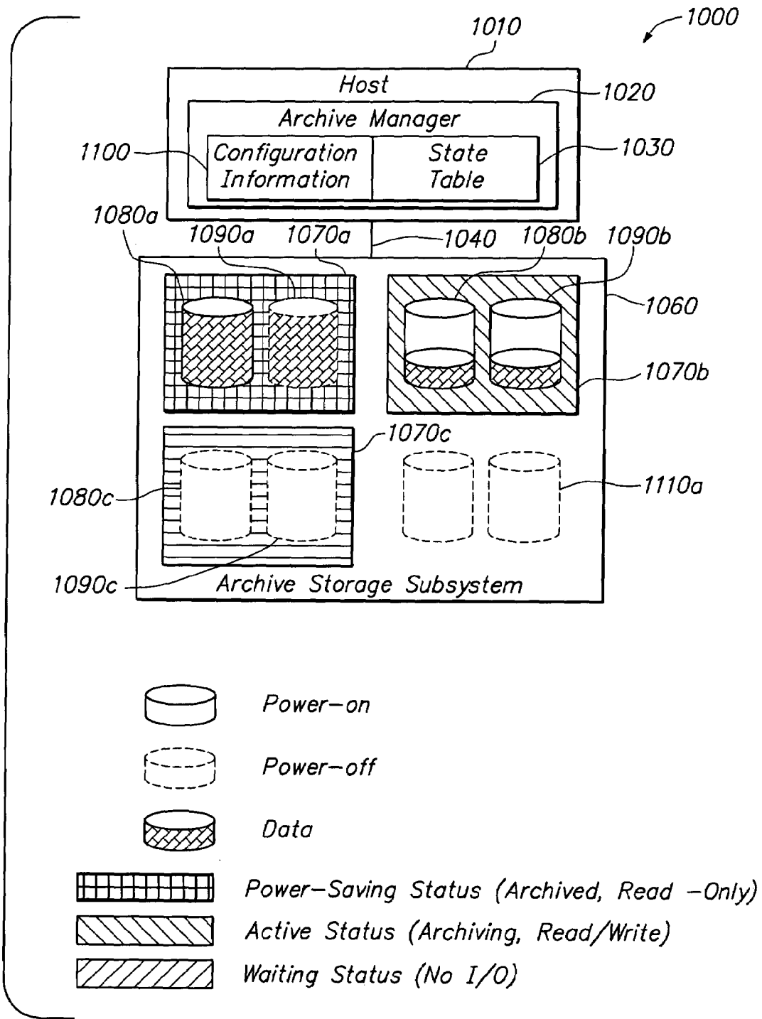
FIG. 3 Status of RAID1
