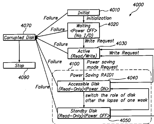
State Transition Diagram (default)
