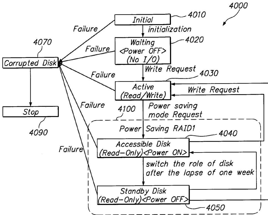
FIG. 6 State Transition Diagram (default)
