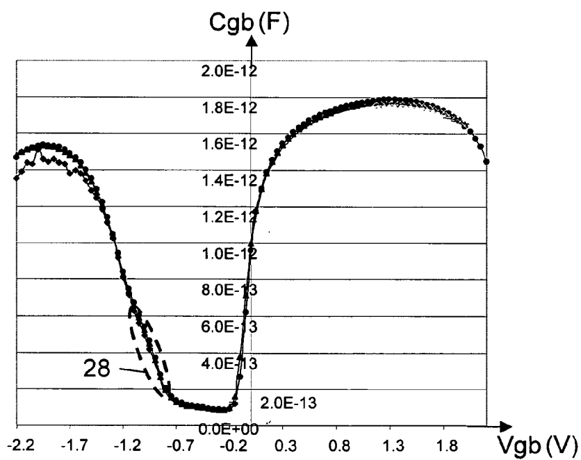
Figure 1 – PRIOR ART
