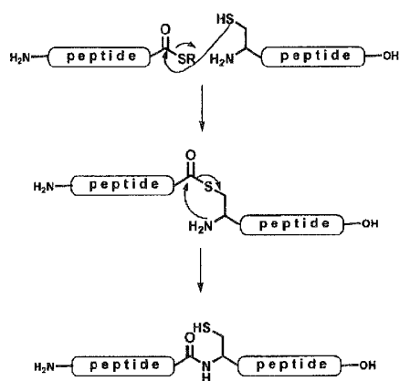
Native Chemical Ligation Method
