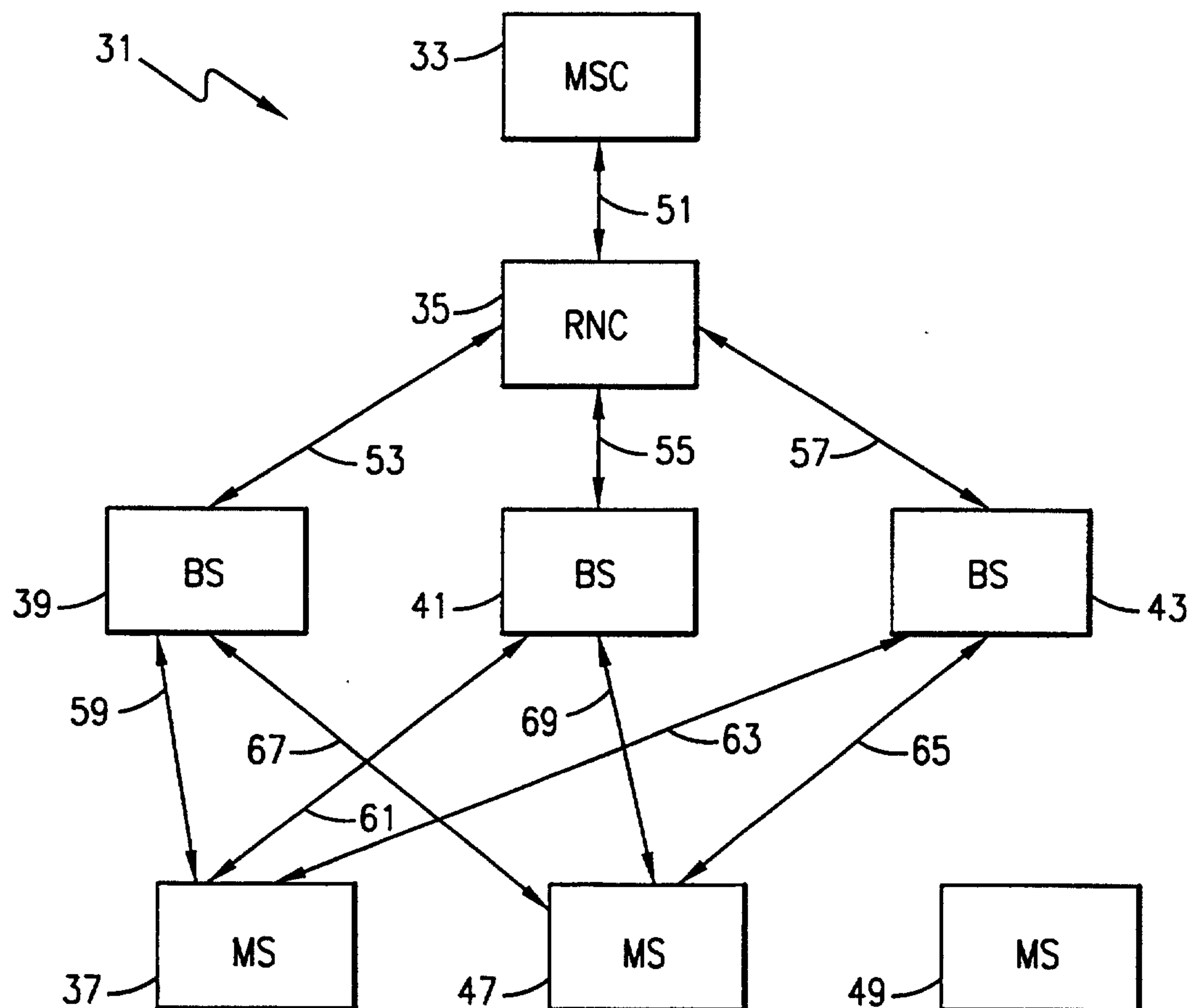
FIG. 2 (PRIOR ART)
