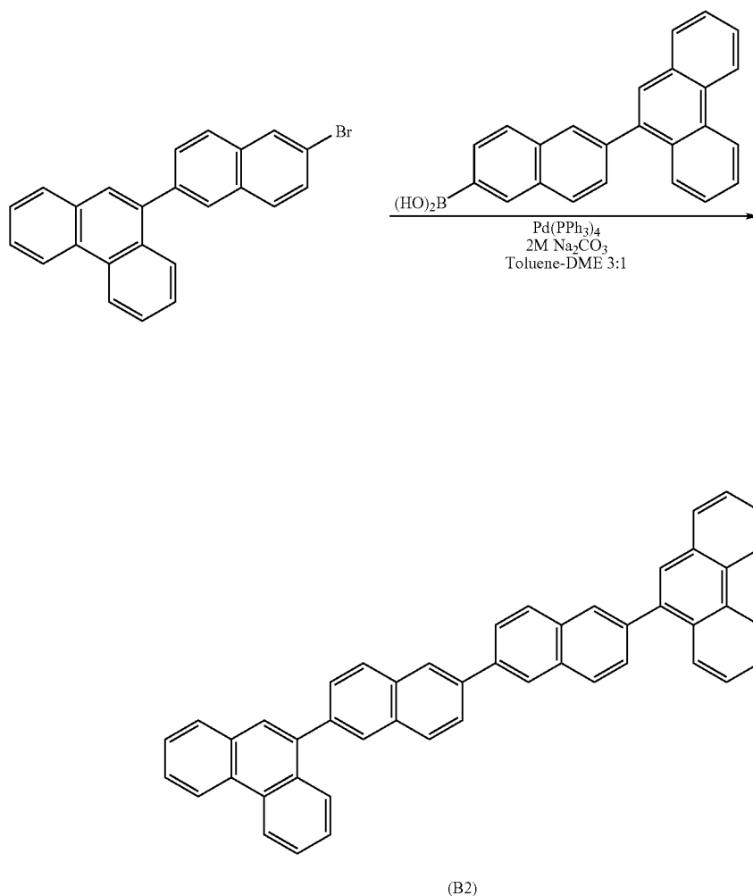
Synthesis of Compound B2
