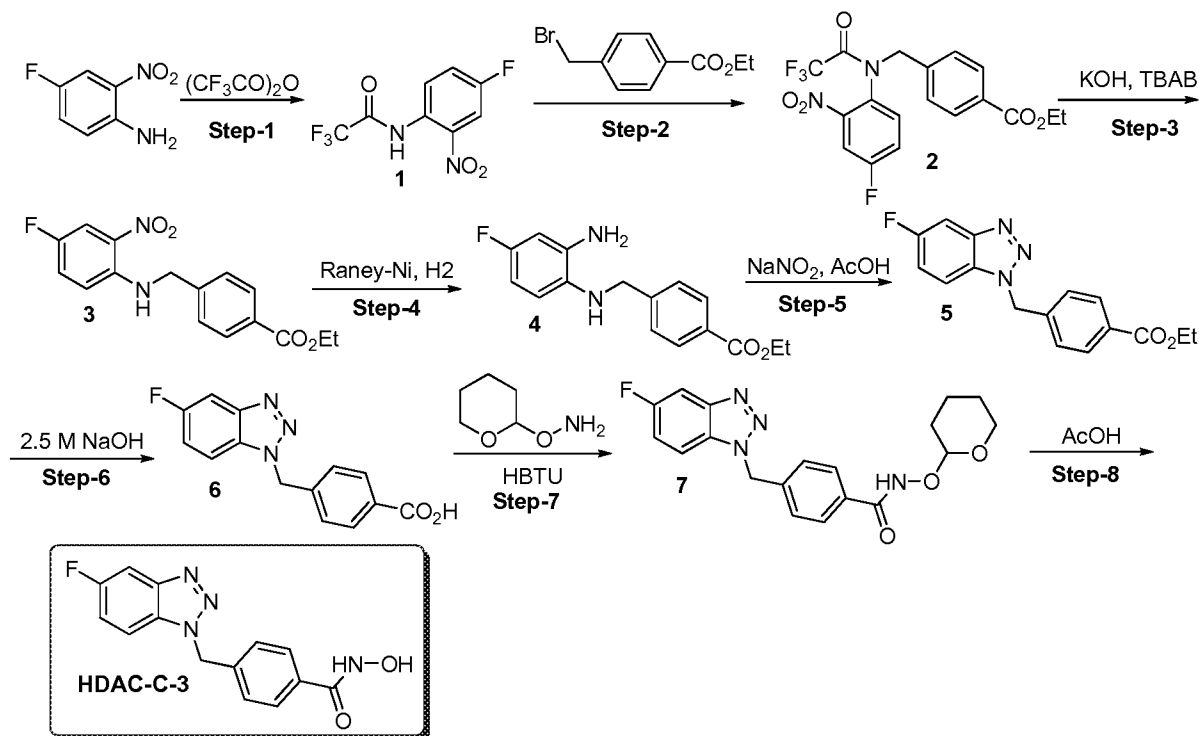
Scheme 3: Synthetic scheme for preparation of HDAC-C-3
