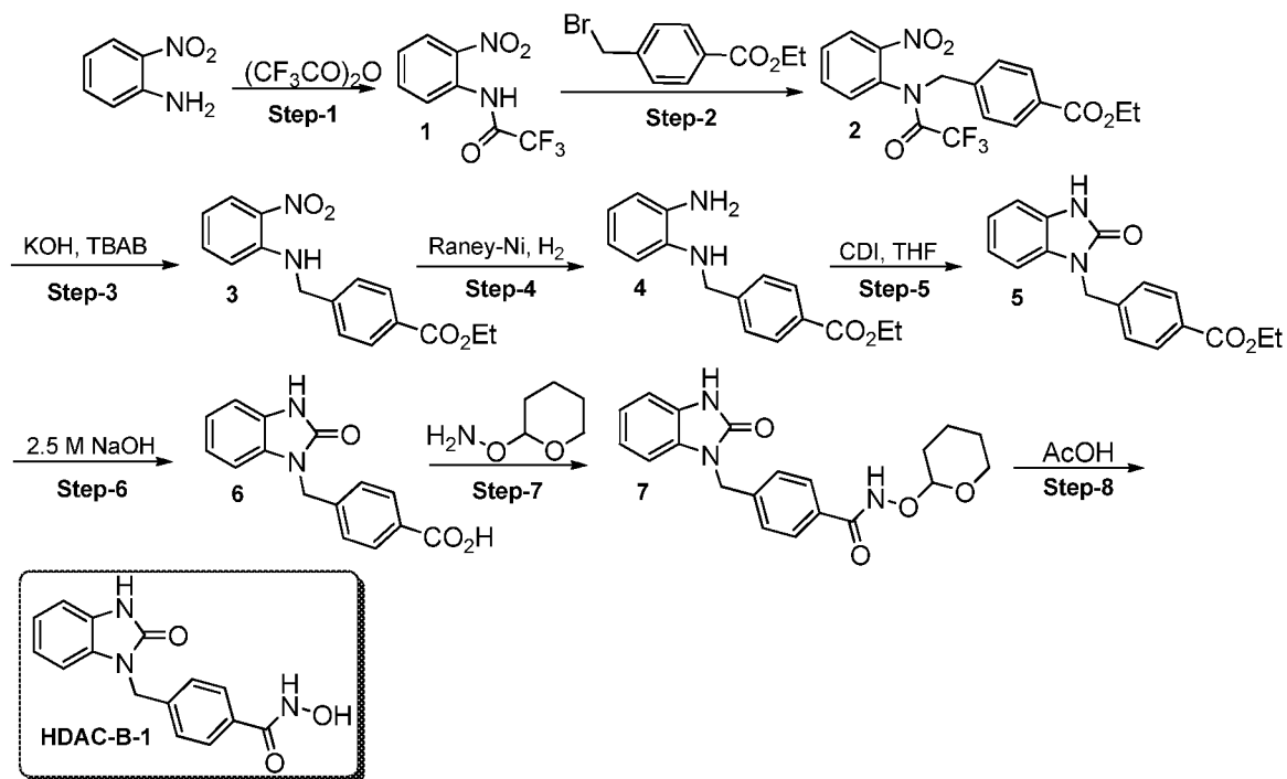
Scheme 2: Synthetic scheme for preparation of HDAC-B1
