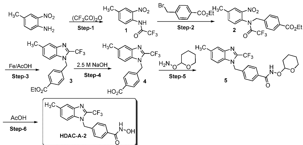
Scheme 1: Synthetic scheme for preparation of HDAC-A2
