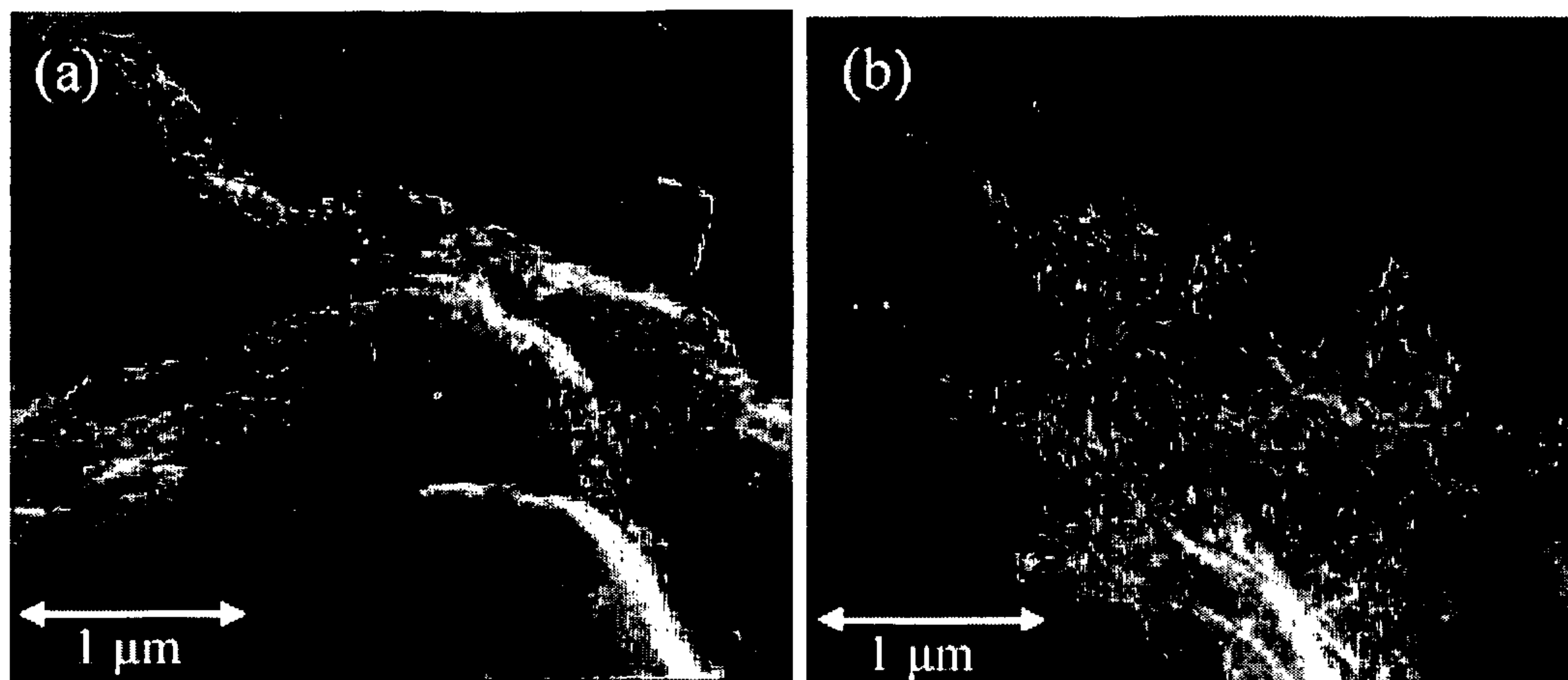
Fig.3: SEM image of carbon nanotubes; (a) before plasma treatment; (b) after plasma treatment for 3 min
