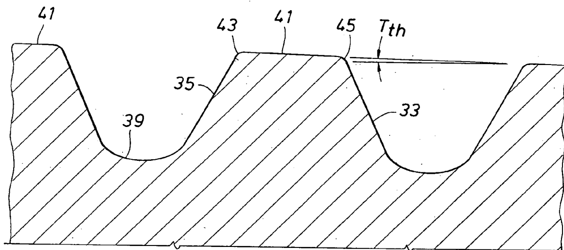
FIG. 5 (PRIOR ART)
