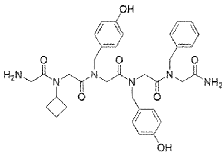
[Chemical Formula 1-3]
