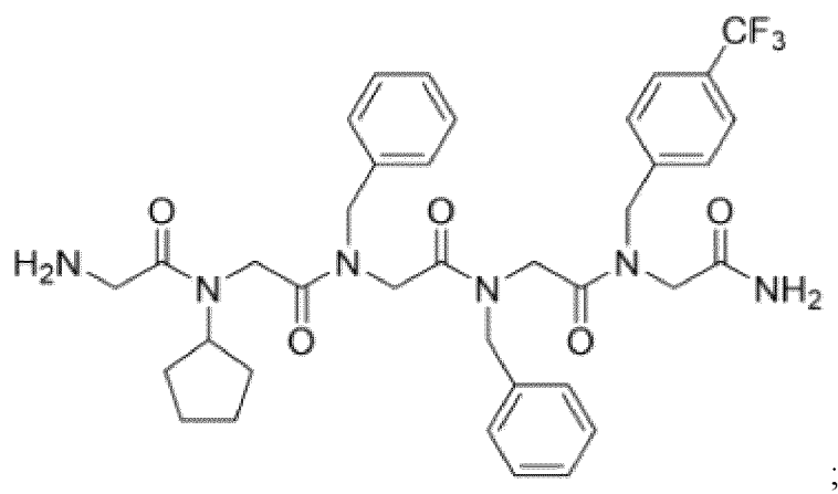
[Chemical Formula 1-16]
