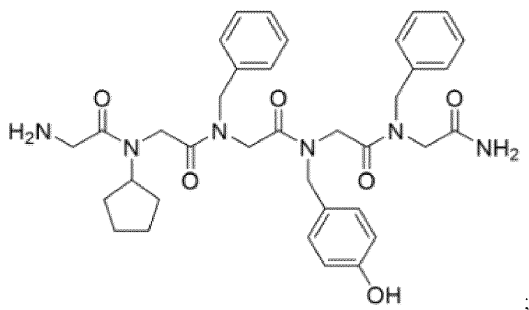
[Chemical Formula 1-9]
