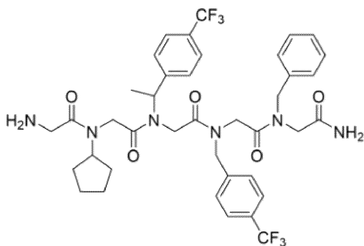
[Chemical Formula 1-18]
