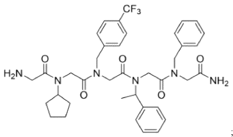
[Chemical Formula 1-17]
