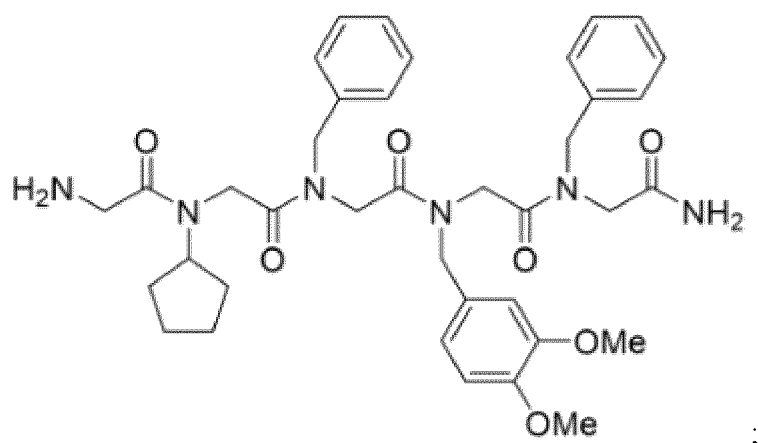
[Chemical Formula 1-15]
