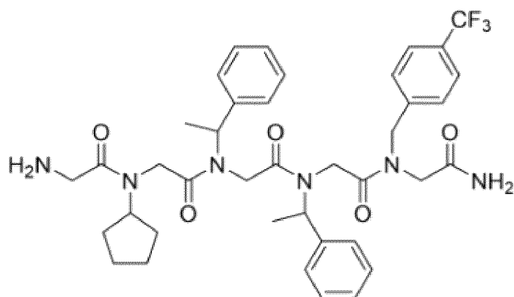
[Chemical Formula 1-19]
