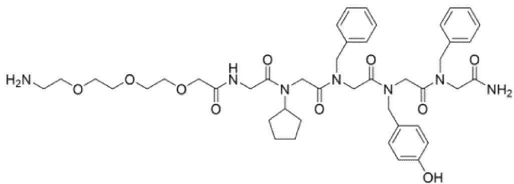
[Chemical Formula 1-26]
