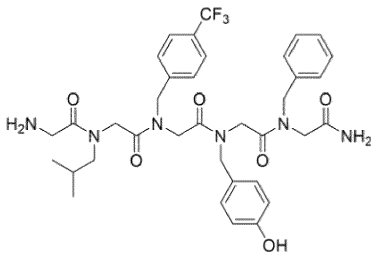
[Chemical Formula 1-8]
