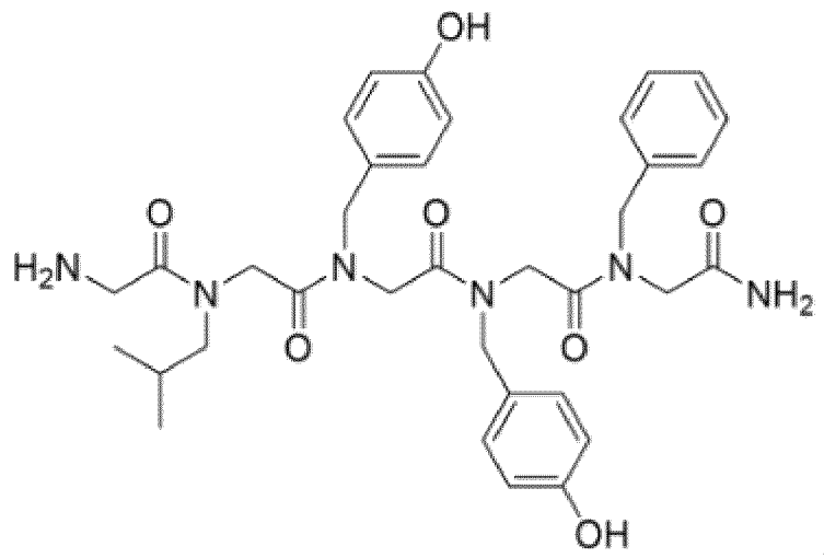
[Chemical Formula 1-2]
