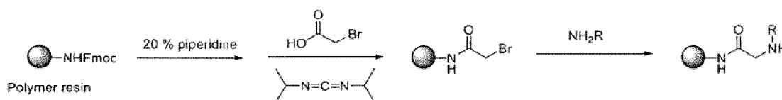
[Reaction Formula 1]
