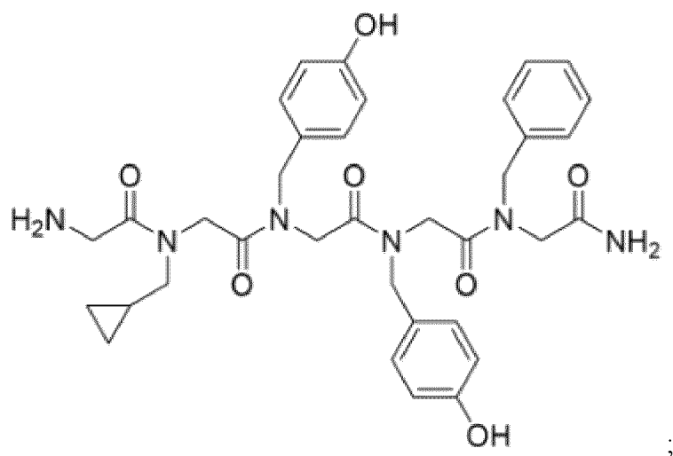
[Chemical Formula 1-11]
