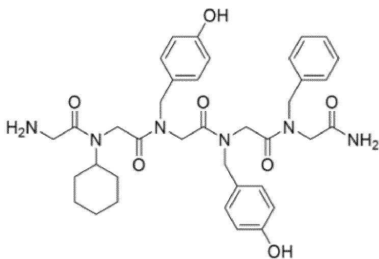
[Chemical Formula 1-12]
