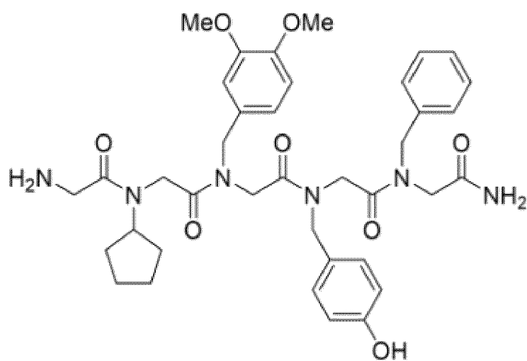
[Chemical Formula 1-13]
