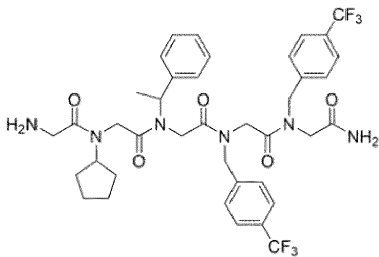
[Chemical Formula 1-20]
