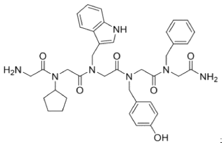
[Chemical Formula 1-11]
