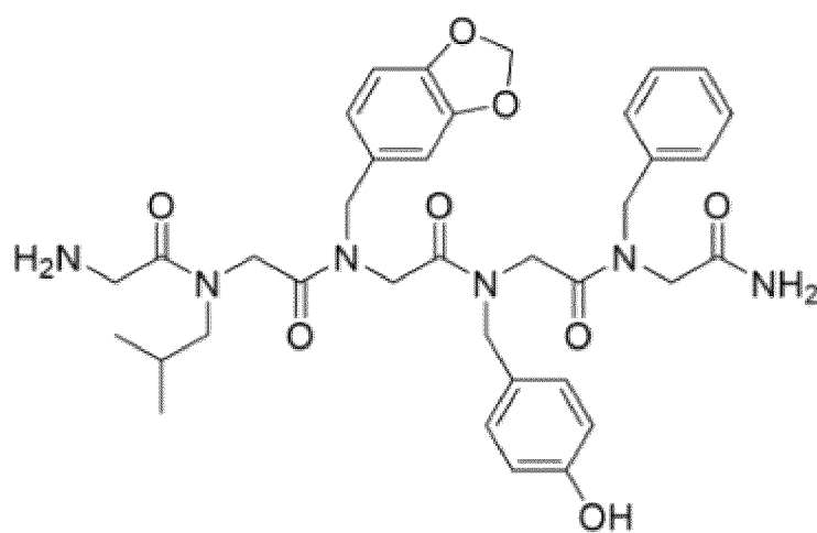
[Chemical Formula 1-6]
