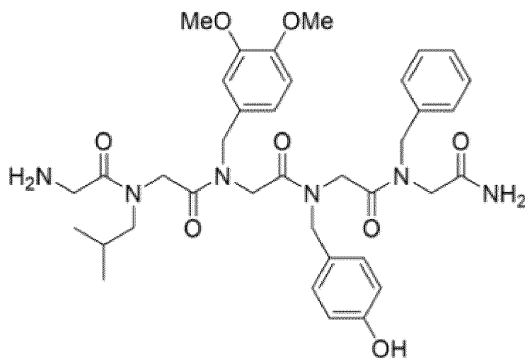
[Chemical Formula 1-7]
