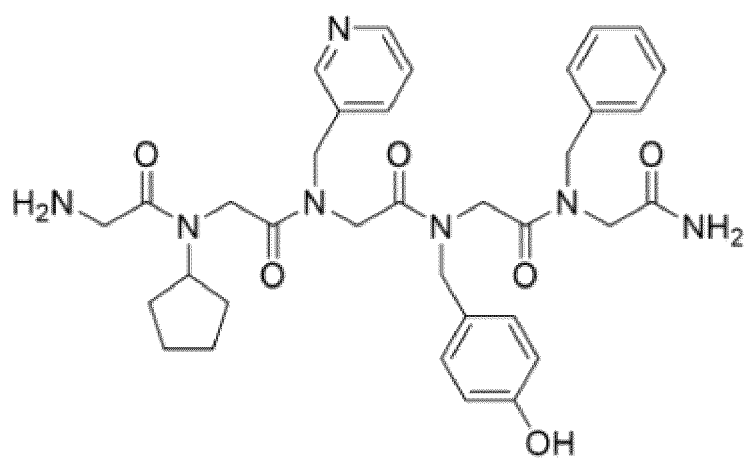
[Chemical Formula 1-24]
