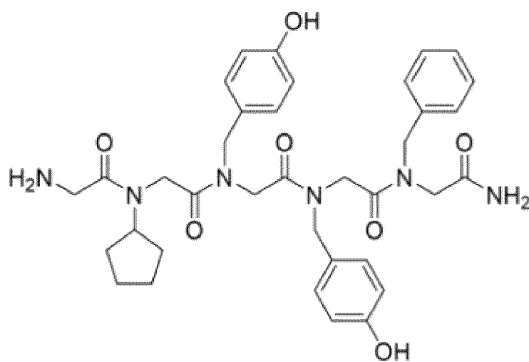
[Chemical Formula 1-4]
