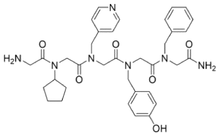
[Chemical Formula 1-25]
