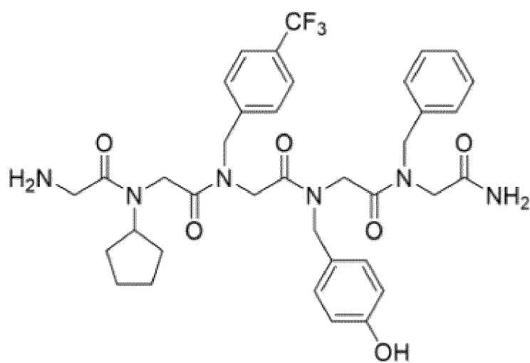
[Chemical Formula 1-14]
