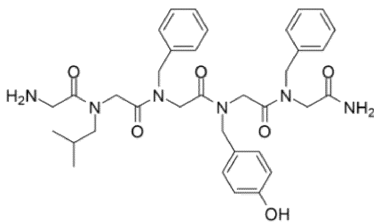
[Chemical Formula 1-5]
