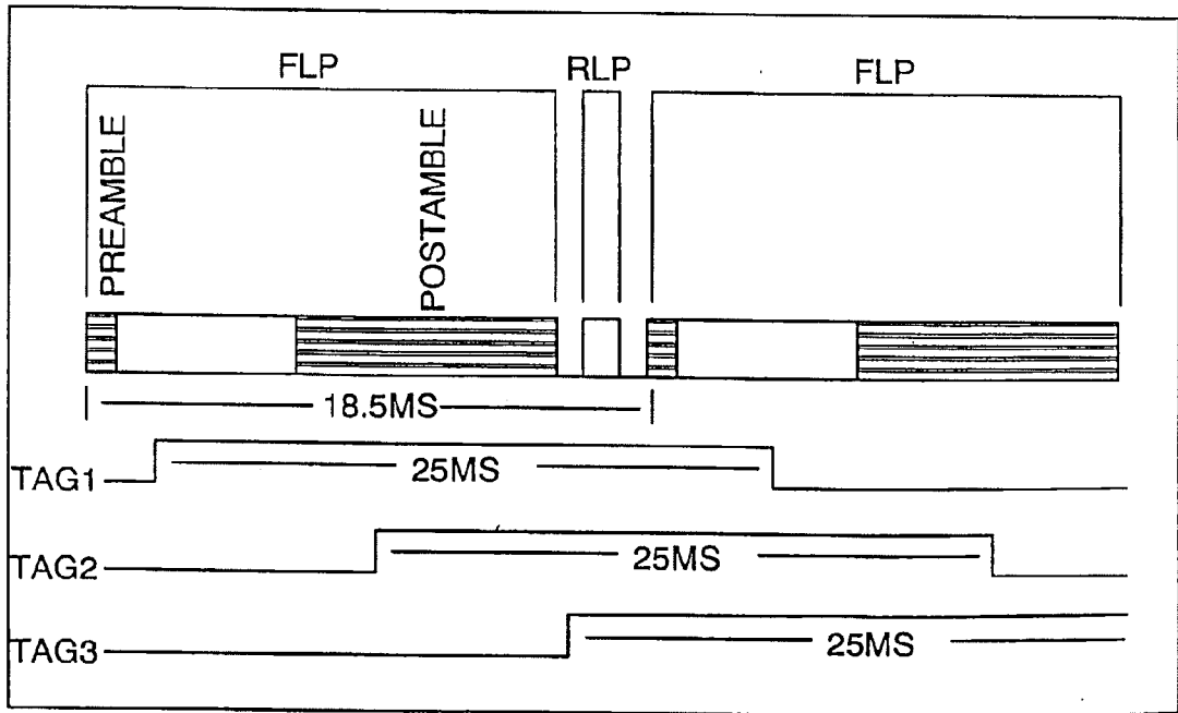
TAG RECEIVER WAKEUP
