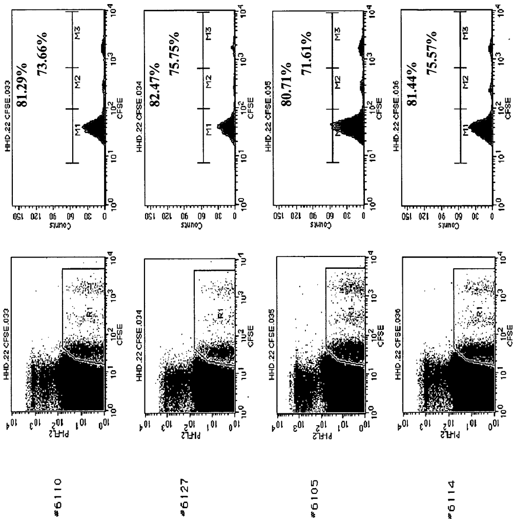
Figure 15C: (L158Nva, C165V) L158Nva C165V NYESO
