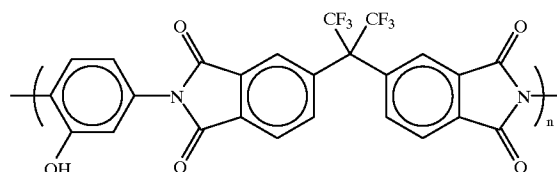
Structure III
