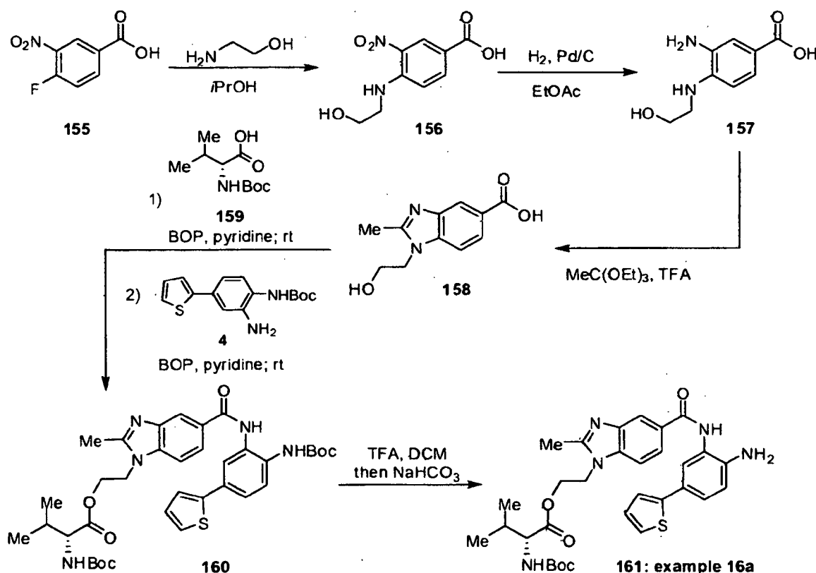
Scheme 16
