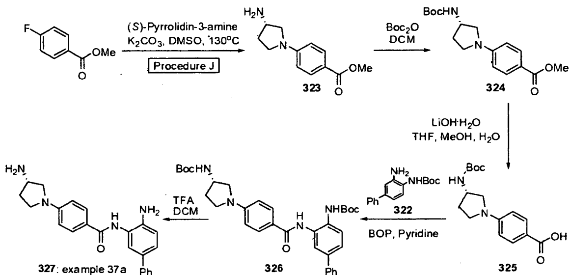
Scheme 37
