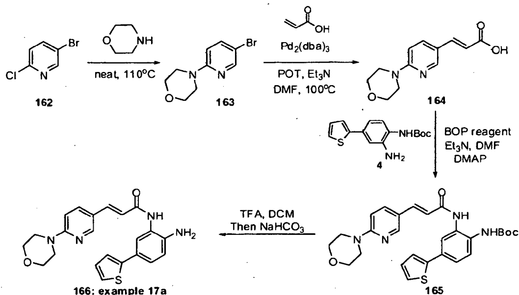
Scheme 17
