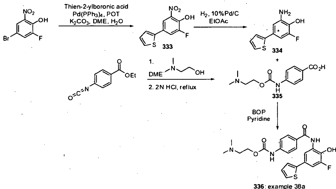
Scheme 38
