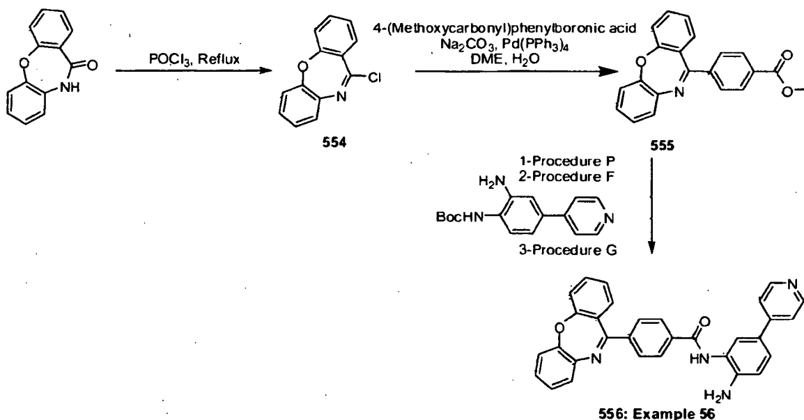
Scheme 56
