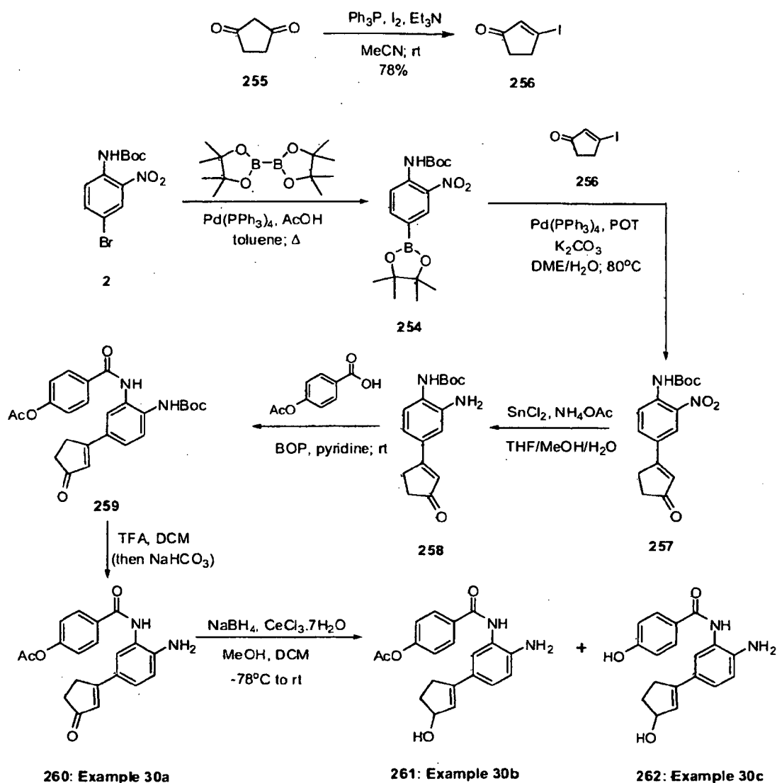
Scheme 30
