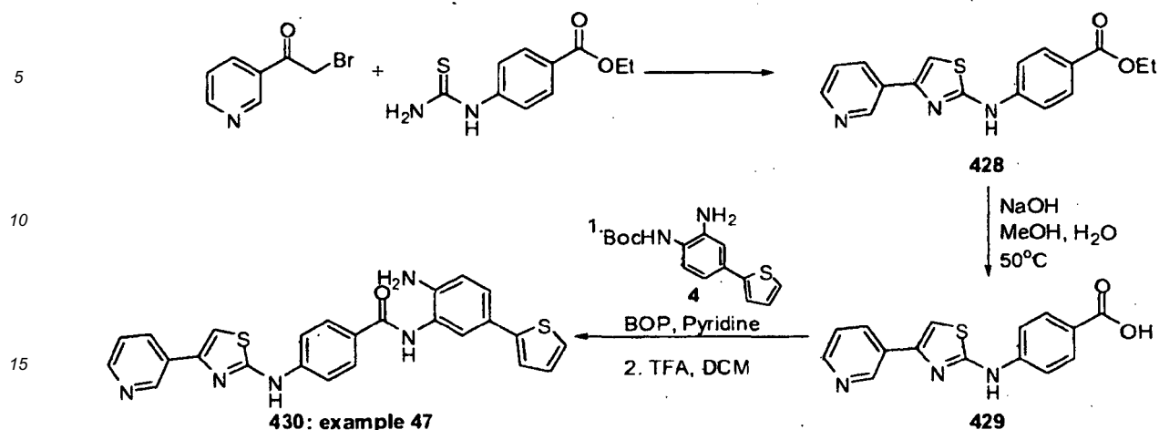
Scheme 47
