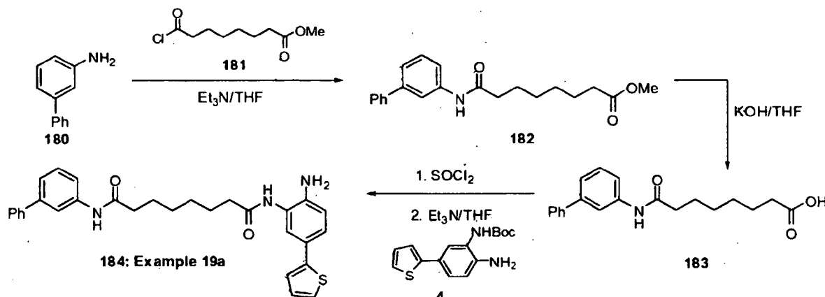
Scheme 19
