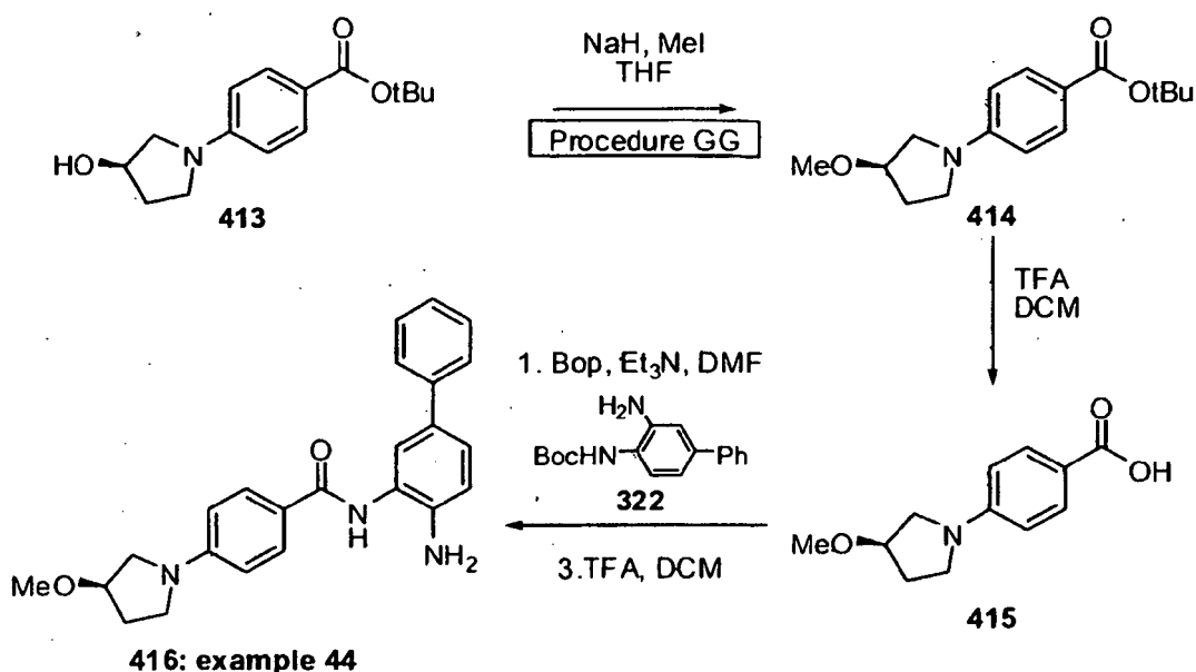
Scheme 44
