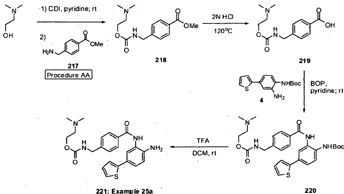
Scheme 25
