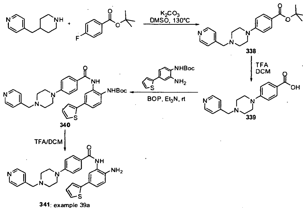
Scheme 39
