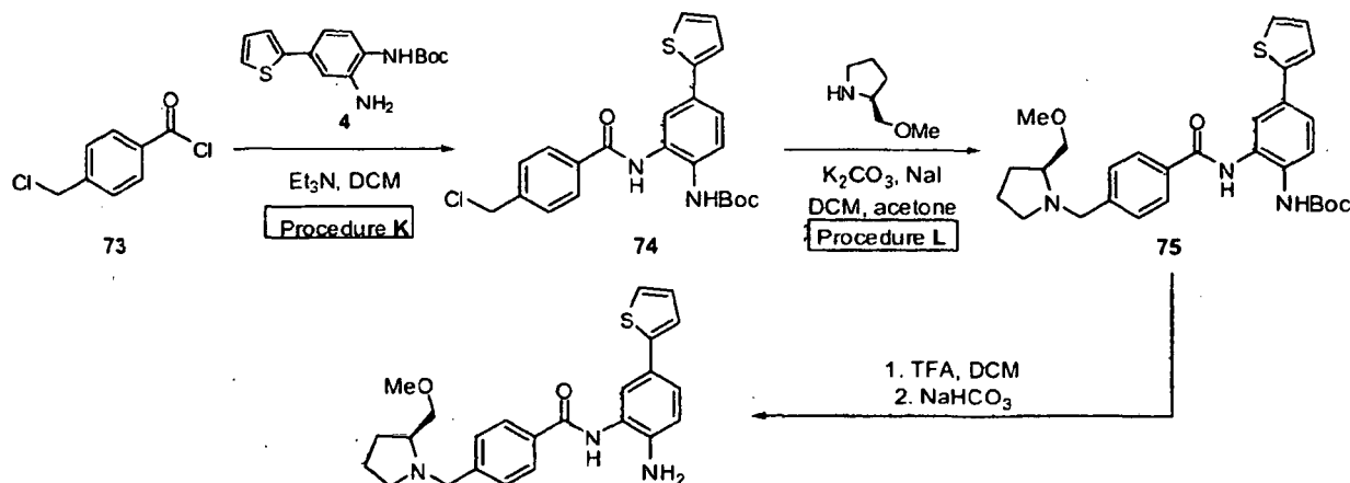
76: example 6a
