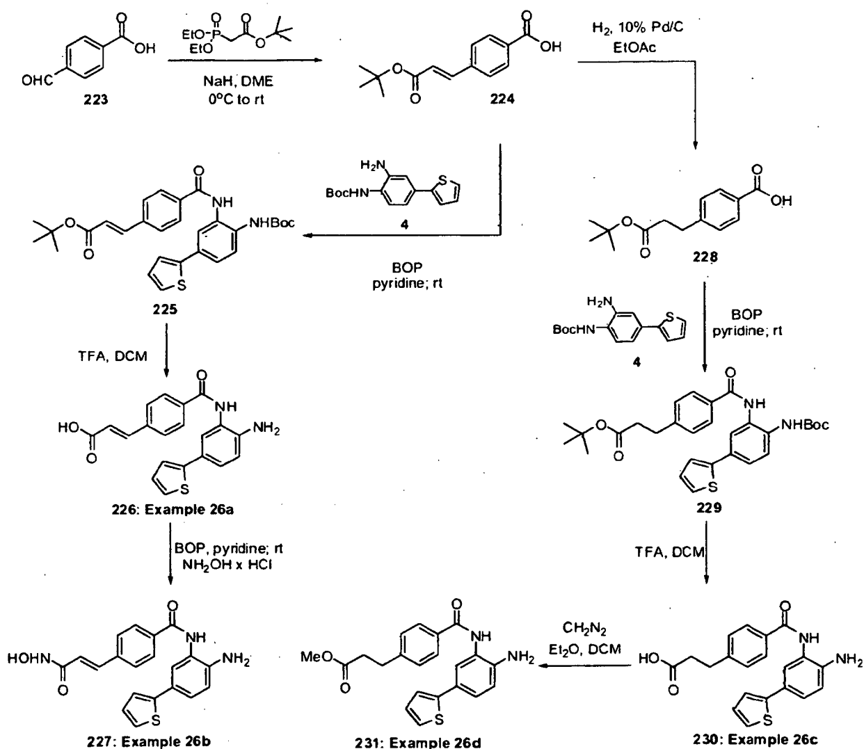
Scheme 26
