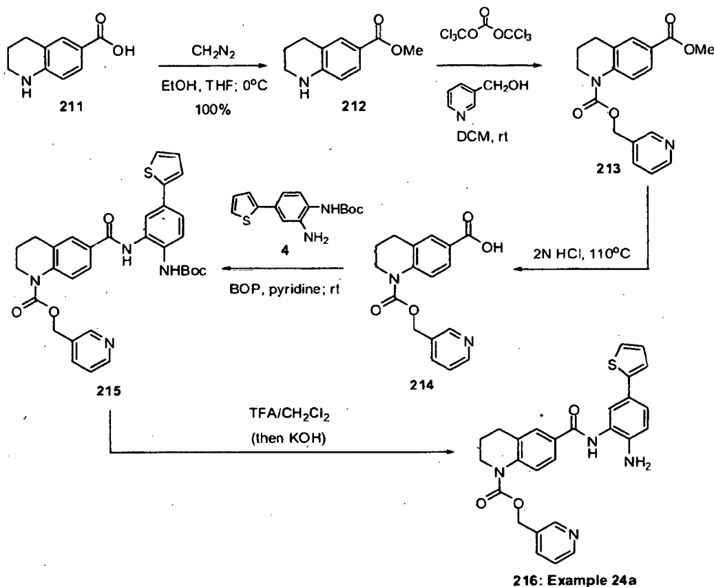
Scheme 24
