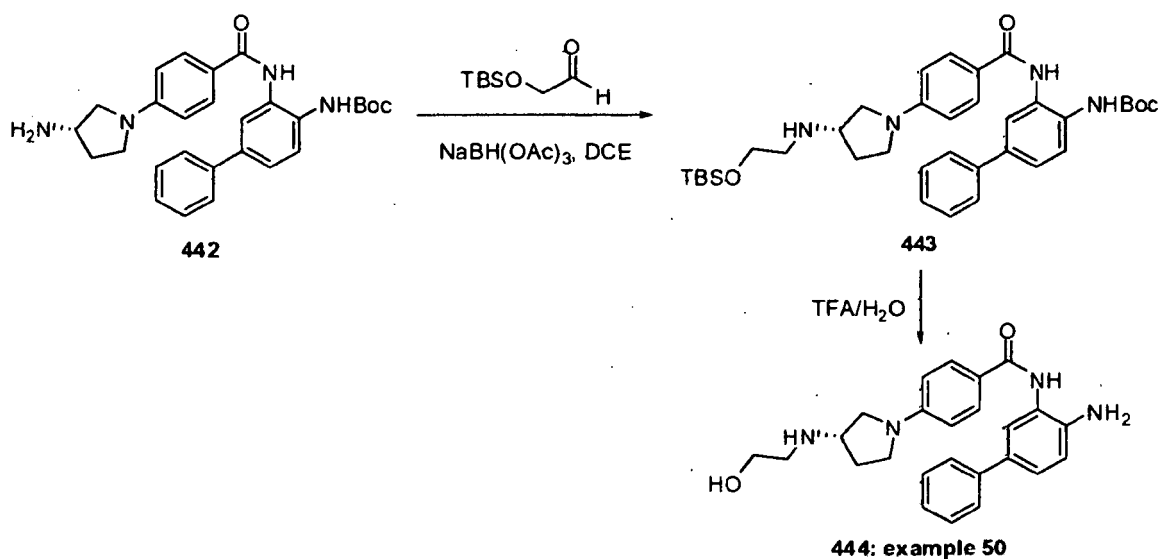
Scheme 50
