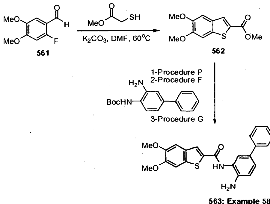
Scheme 58
