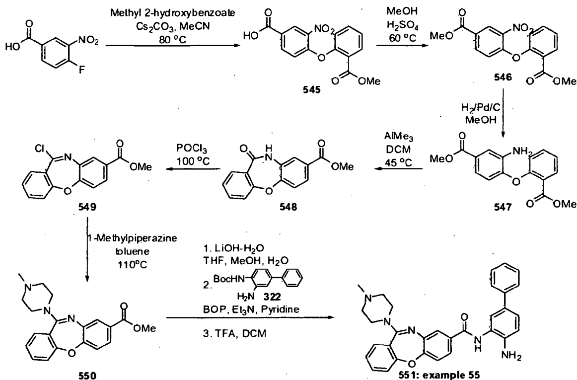
Scheme 55
