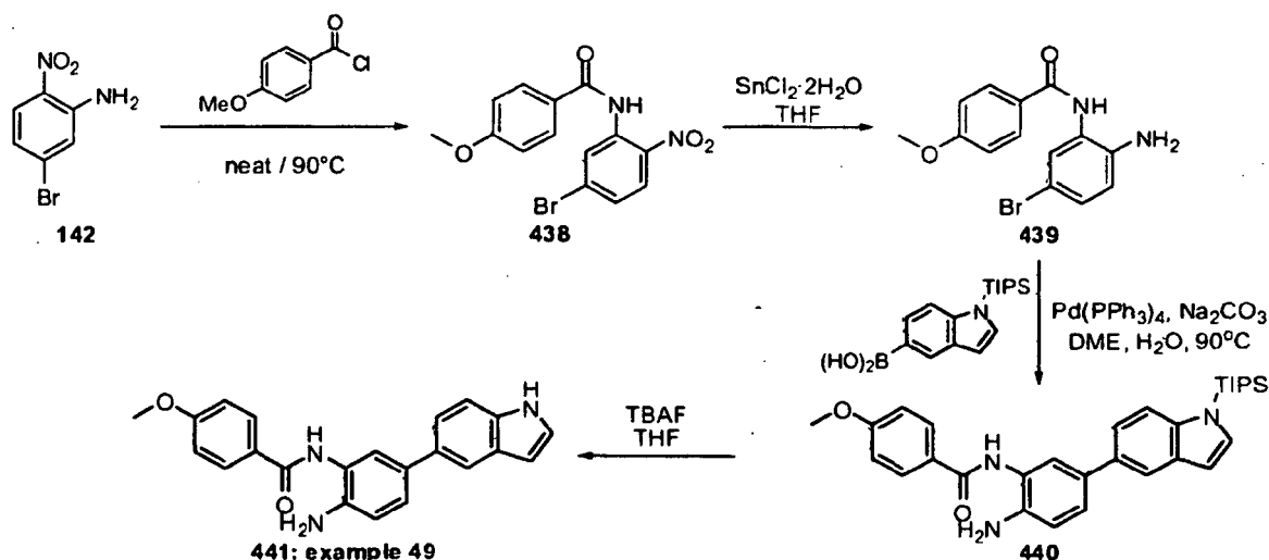
Scheme 49
