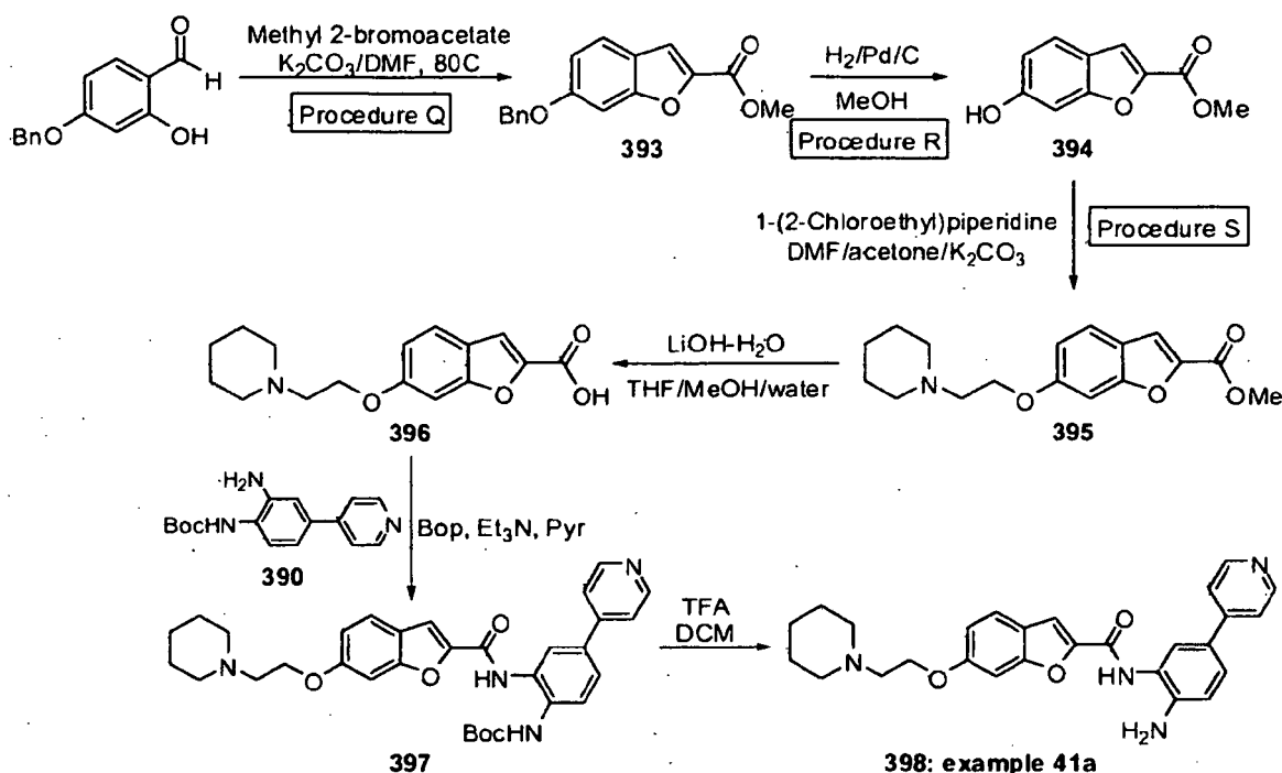
Scheme 41
