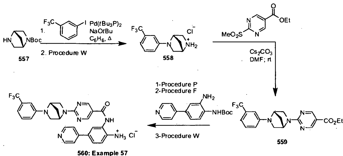
Scheme 57
