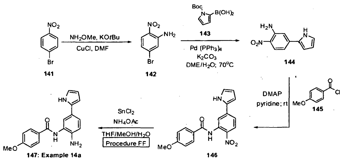
Scheme 14
