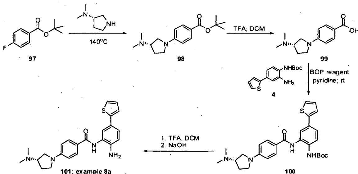
Scheme 8
