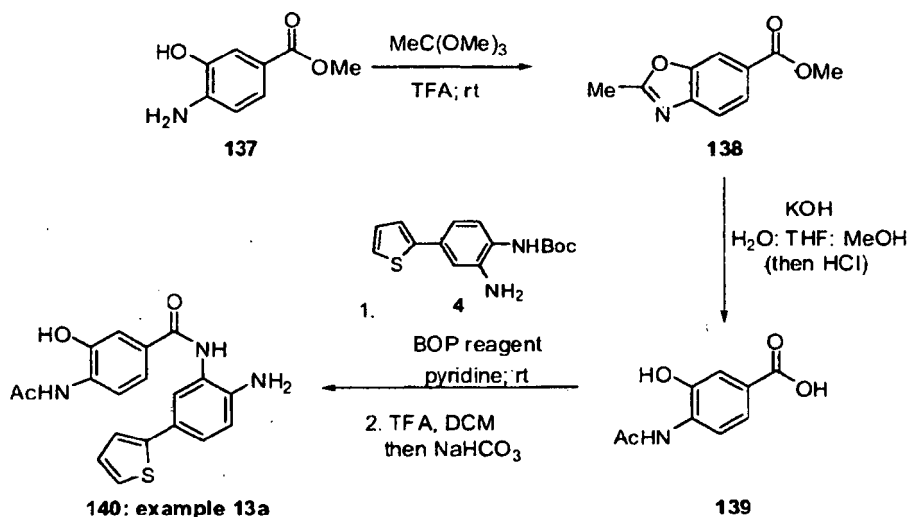
Scheme 13
