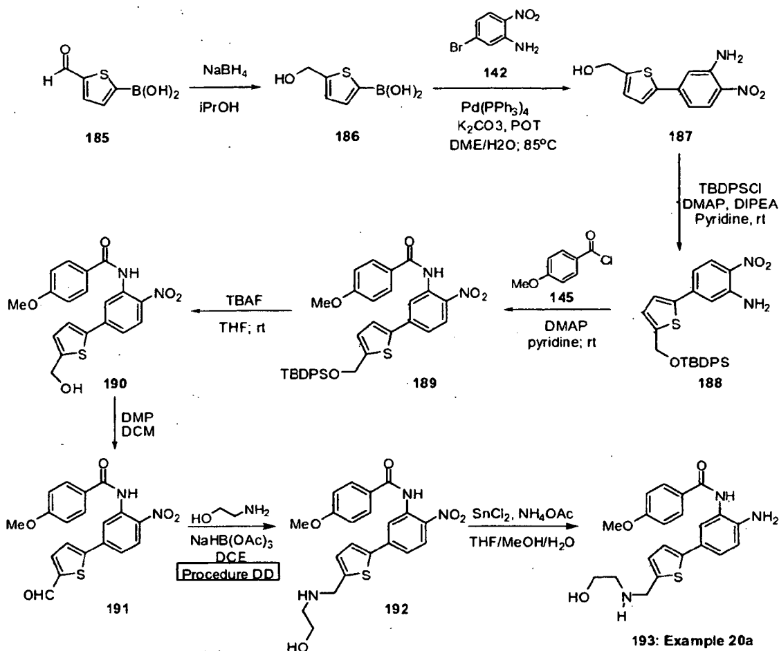
Scheme 20
