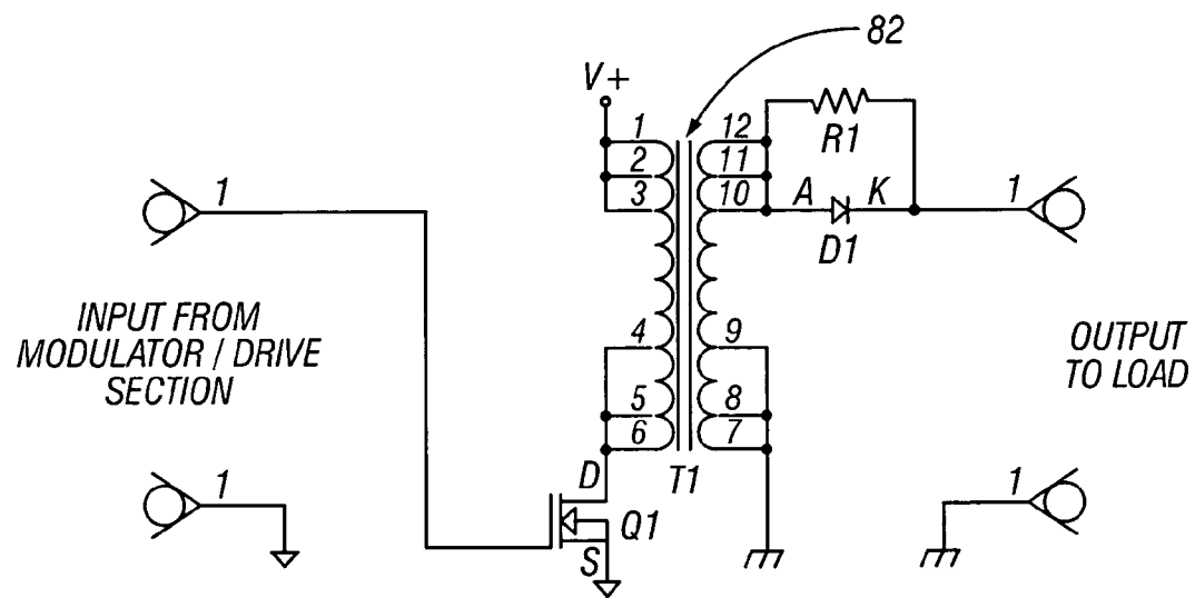
SIMPLIFIED INVERTER SECTION SCHEMATIC
