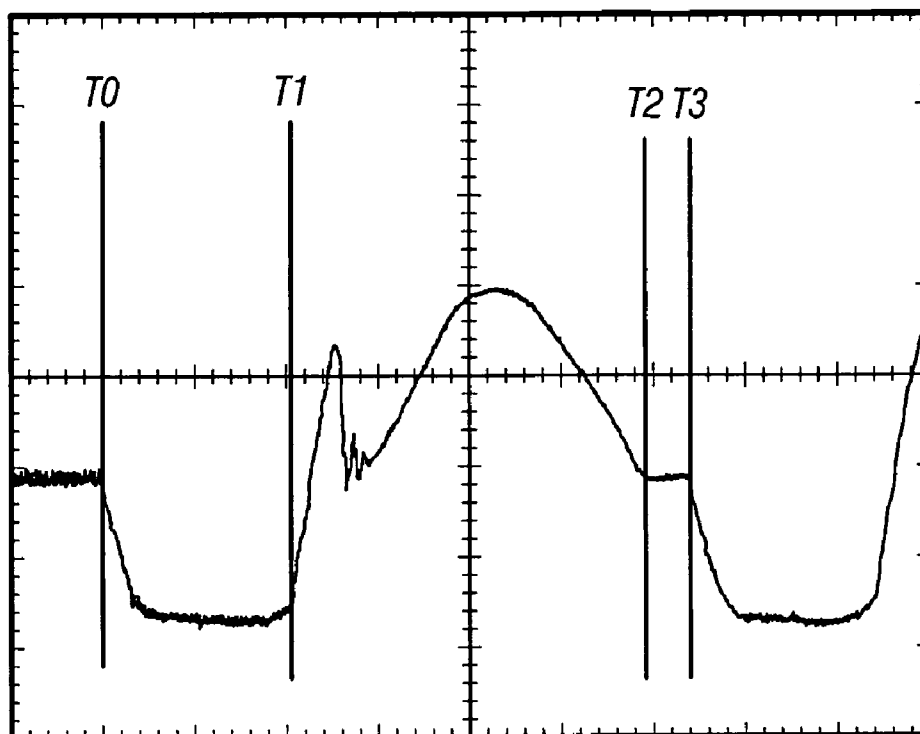
MOSFET Switch Drain Voltage
