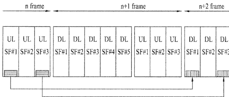
(a) DL/UL ratio 5:3
