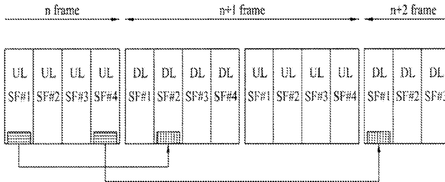
(b) DL/UL ratio 4:4
