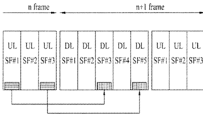
(a) < DL/UL ratio 5:3 >
