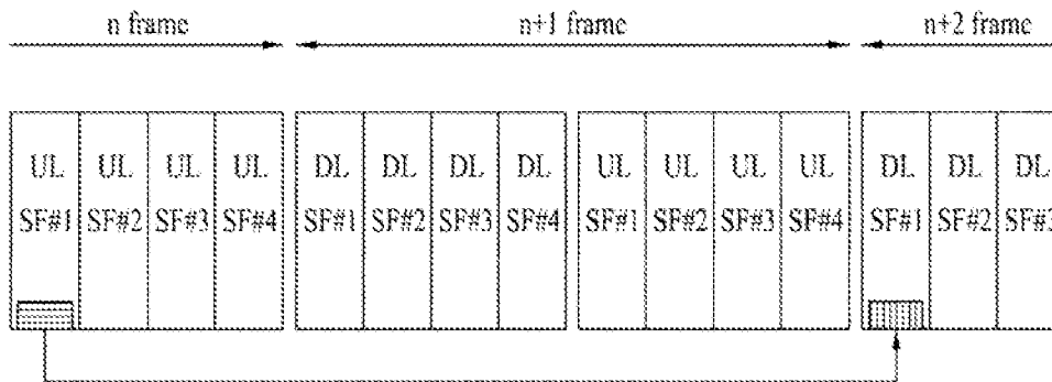
(b) DL/UL ratio 4:4
