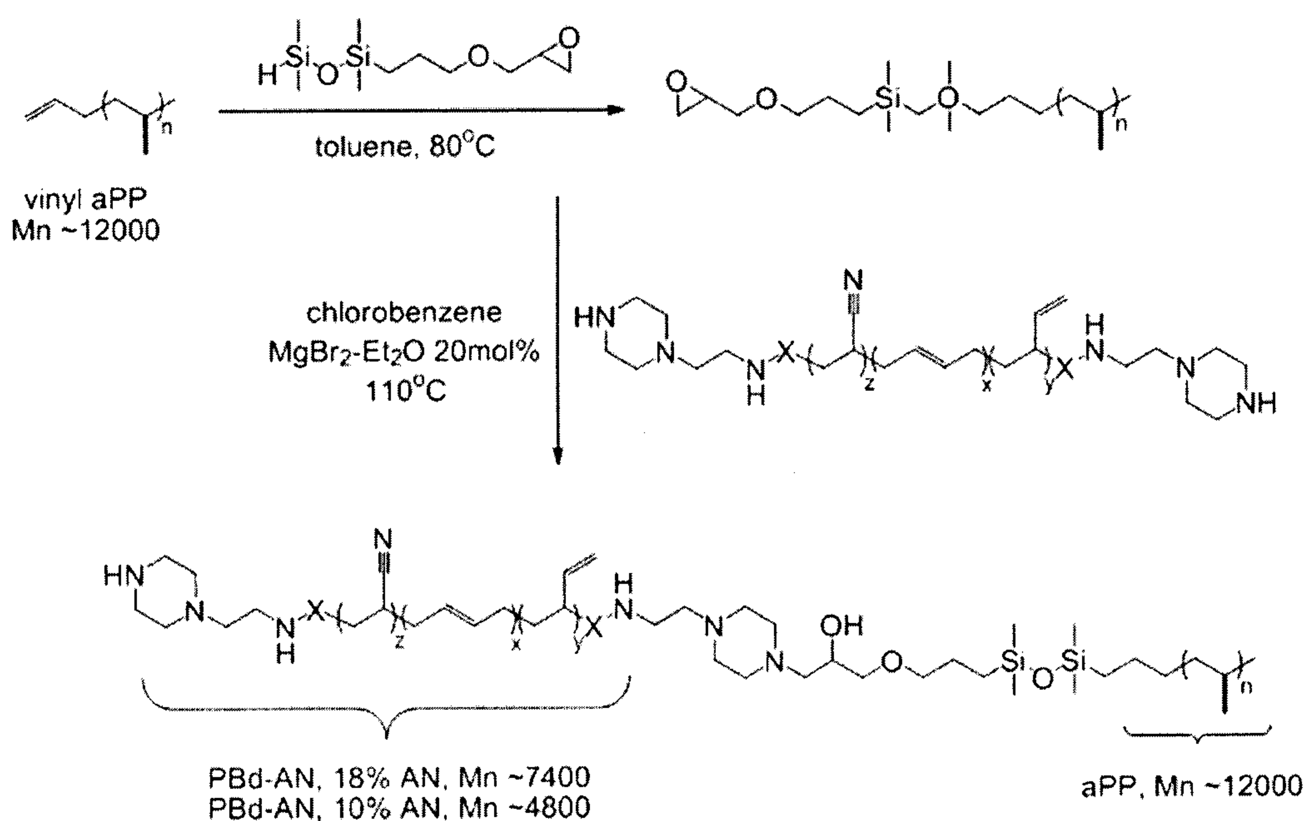
Scheme 3: Reaction between vinyl terminated aPP and poly(butadiene-co-acrylonitrile)-amine.
