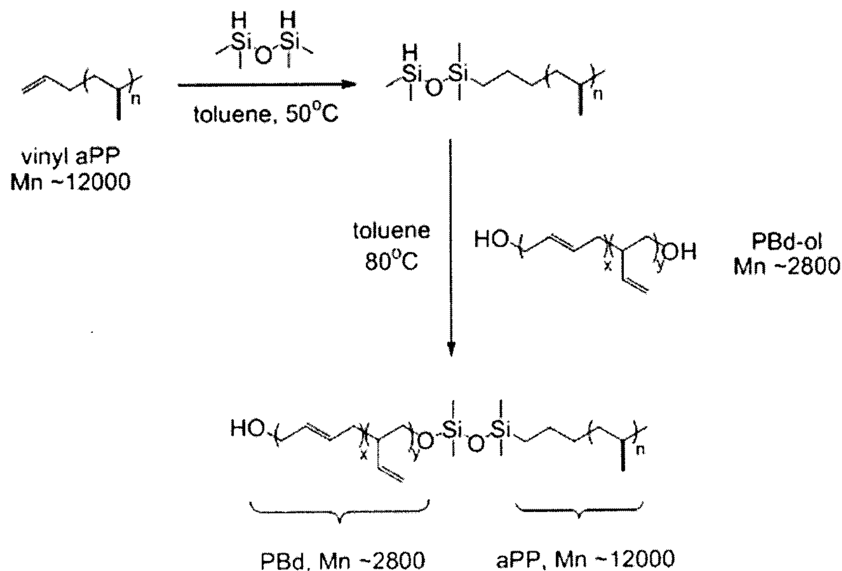
Scheme 2: Reaction between vinyl terminated aPP and polybutadiene diol.
