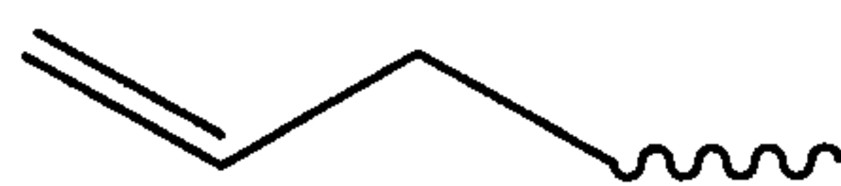
allylic vinyl end group (I)
